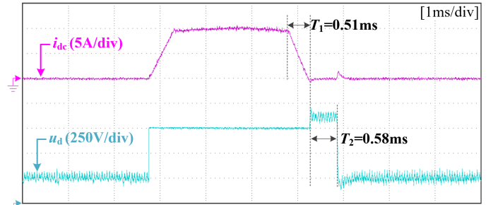
Fig. 14. Experimental waveforms of i_{dc} and u_a at 10 Hz under full-torque.
