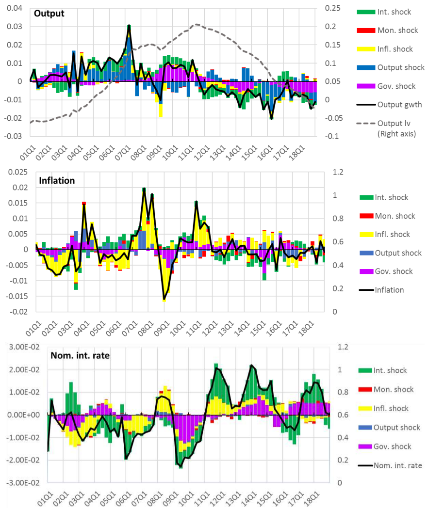
Figure 5: Historical decomposition
