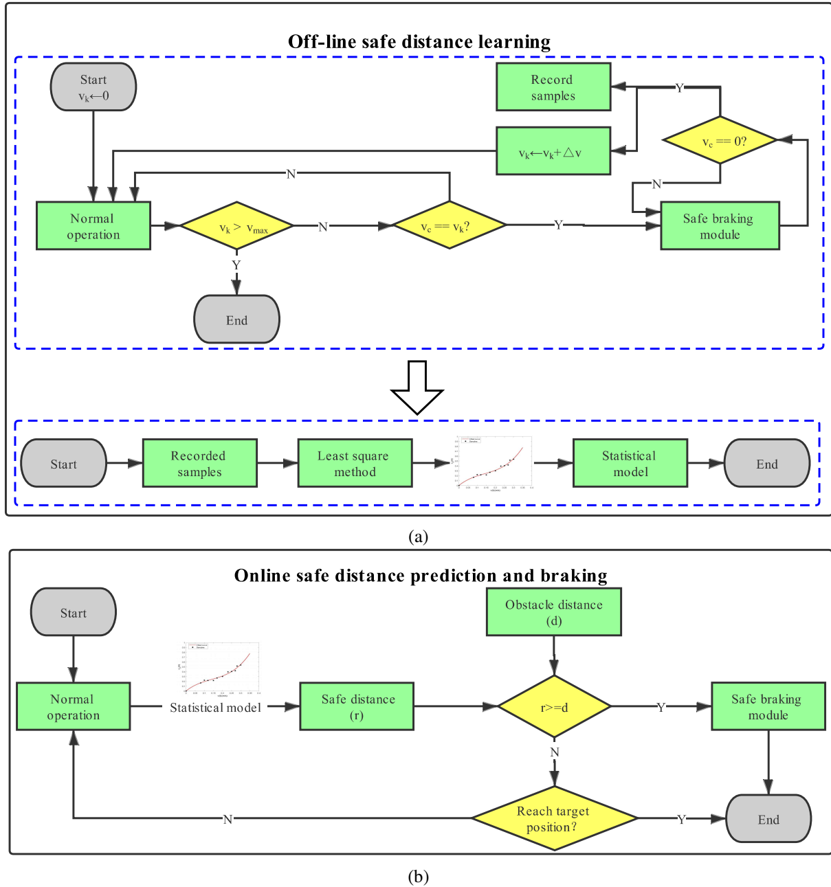
FIGURE 3 The flow chart of model prediction control (MPC) method for safe distance learning (a) and braking with anti-swing (b). For off-line safe distance learning, we try to find different braking distances with different initial velocities using the proposed MPC anti-swing control algorithm, where v_c represents the current velocity, v_k is a predefined velocity sample and v_{max} is the maximum limitation of the crane. In each iteration, the crane starts from zero velocity and accelerates (normal operation) until the current speed v_c is equal to v_k . Then, the safe braking module starts to work until the crane stops. The braking distance is then recorded with respect to different v_k , which is updated with a step size of \Delta v . After these samples are recorded, the least square method is used to find the statistical model between the initial velocities and safe braking distances. For online safe distance prediction and braking, we compare the safe braking distance and the distance to the obstacle to decide whether the crane is safe to continues or not.
