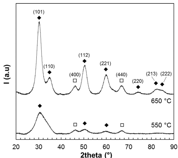
Fig. 2. XRD patterns of YSZ- \gamma -Al 2 O 3 powders (50 wt% YSZ) calcined in air at 550 °C and 650 °C for 3 h. (◆): (ZrO 2 ) 0.92 (Y 2 O 3 ) 0.08 (JCPDS 01-070-4431); (□) Gamma-Al 2 O 3 (JCPDS 00-002-1420).
