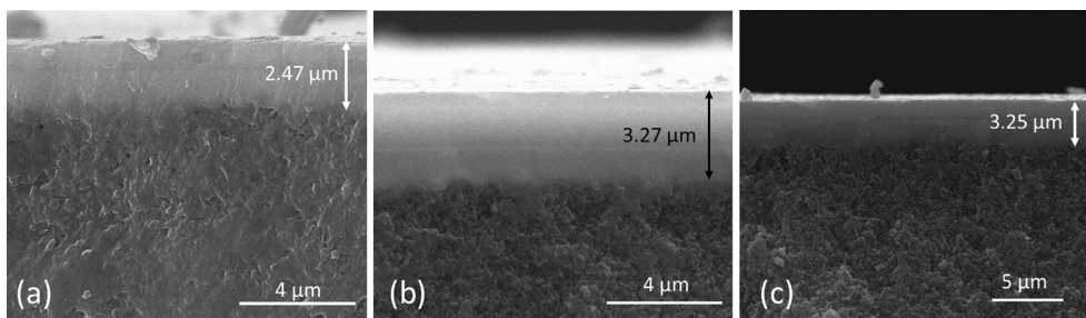
Fig. 4. SEM cross section images of PF-A133 (a), PF-145 (b) and PF-155 (c).
