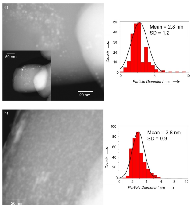
Figure 2. HAADF-STEM micrographs and corresponding histogram plots of the reduced a) Pt/Silicalite-1 sample, and b) Pt/Sn-Silicalite-1 catalysts.
