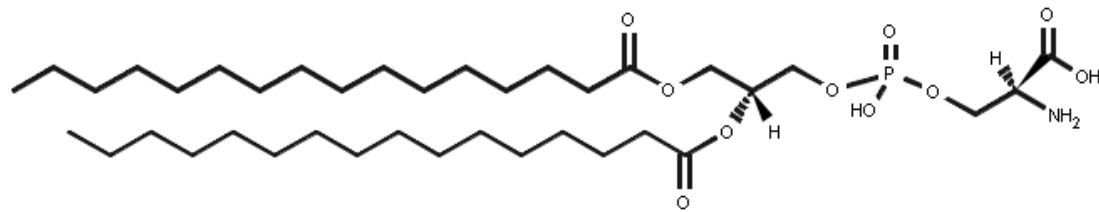
Phosphatidylserine
