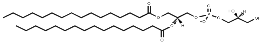
Phosphatidylglycerol
