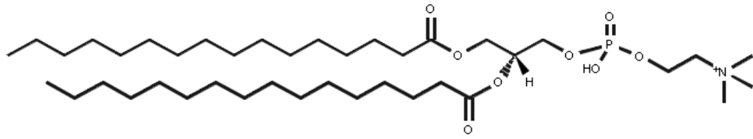
Phosphatidylcholine
