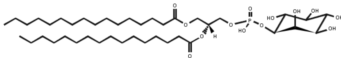
Phosphatidylinositol
