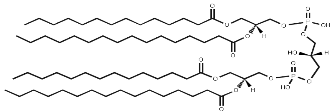
Diphosphatidylglycerol (cardiolipin)
