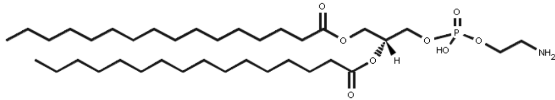
Phosphatidylethanolamine
