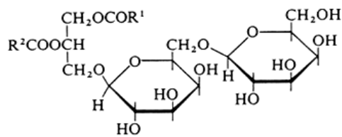
Digalactosyldiacylglycerol
