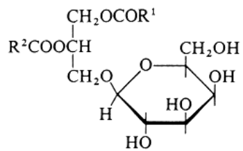
Monogalactosyldiacylglycerol
