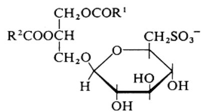
Sulfoquinovosyldiacylglycerol
