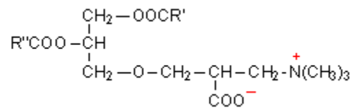
1,2-diacylglyceryl-3-O-2'-(hydroxymethyl)-( N,N,N -trimethyl)- \beta -alanine (DGTA)
