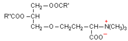
1,2-diacylglyceryl-3-O-4'-( N,N,N -trimethyl)-homoserine (DGTS)
