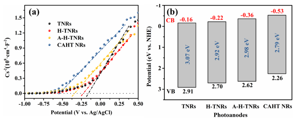
Figure S11. Mott-Schottky plots(three-electrodes cell employing 0.5 M Na 2 SO 4 solution) (a) and relative changes of the CB, Fermi and VB positions (b) of as-prepared films.
