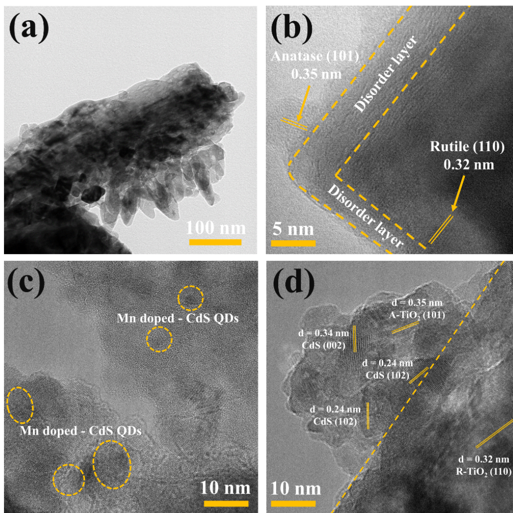
Figure 3. TEM image (a) and HRTEM images (b-d) of CAHT NRs composite films.
