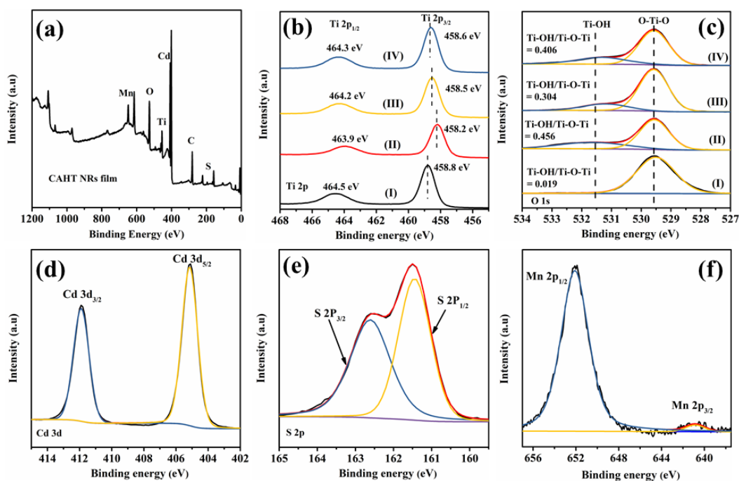
Figure 4. Full scan survey XPS spectrum (a) and exemplified XPS spectra of Ti 2p (b), O 1s (c), Cd 3d (d), S 2p (e) and Mn 2p (f) from quaternary CAHT NRs hybrid composite. A comparison of Ti 2p and O 1s XPS spectra between different samples (TNRs (I), H-TNRs (II), A-H-TNRs (III) and CAHT NRs (IV)) is also listed in (b) and (c), respectively.
