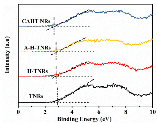
Figure S3. XPS VB spectrum of the as-prepared film.
