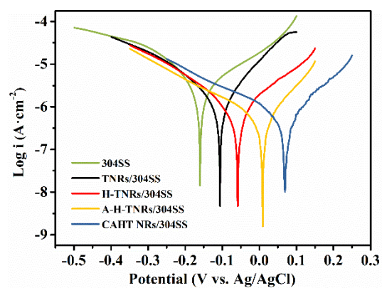
Figure S7. Polarization curves of bare 304SS, and 304SS in 3.5 wt% NaCl solution coupled with different photoanodes in 0.1 M Na 2 S and 0.2 M NaOH mixed solution in the dark condition.
