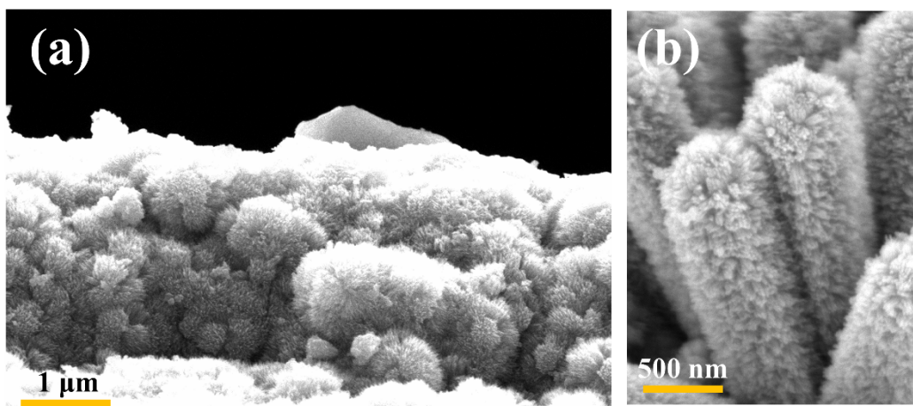
Figure S1. Cross-section SEM images of the CAHT NRs composite film (a and b).
