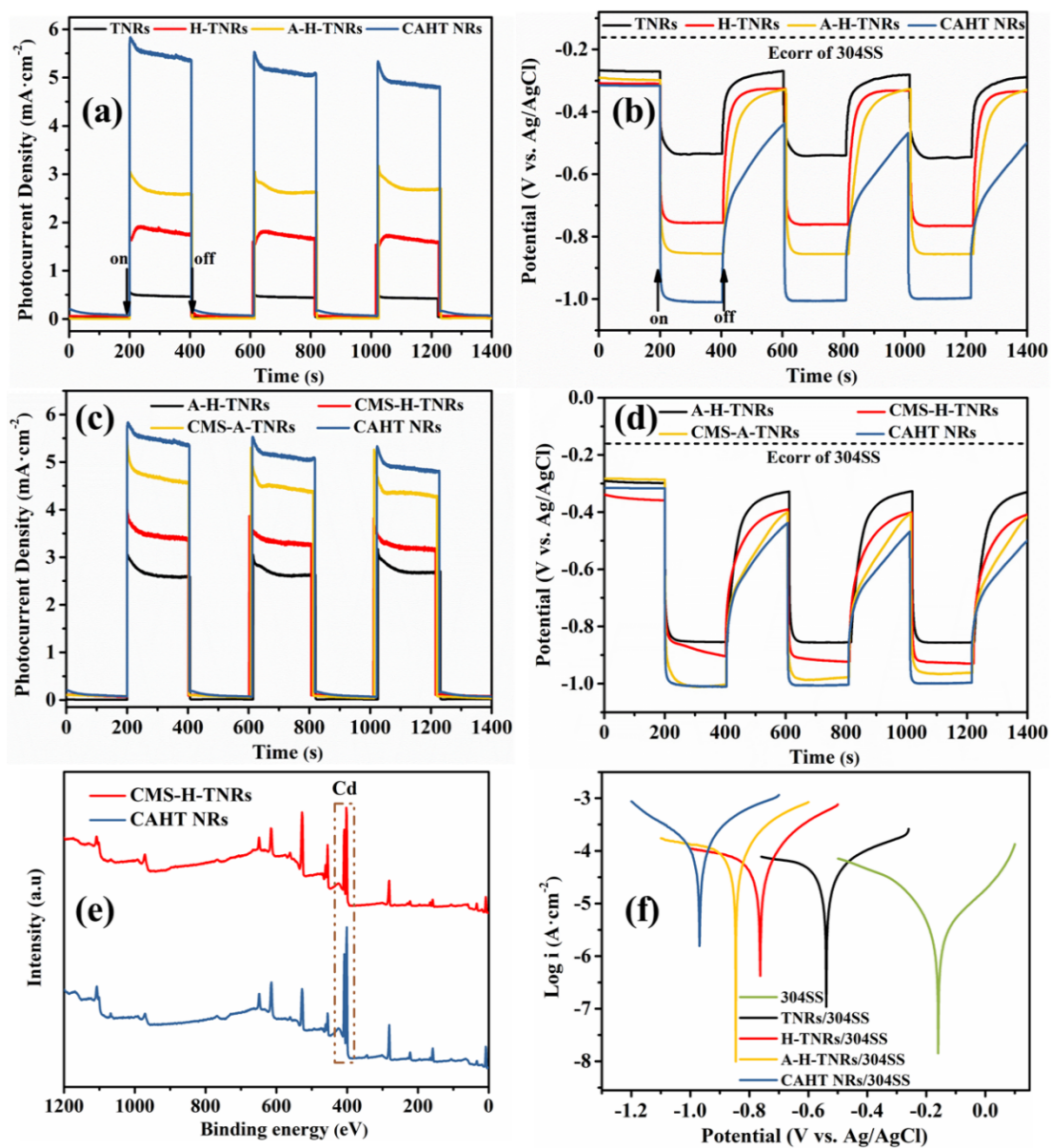
Figure 5. (a and c) The photocurrent responses, (b and d) potential variations, (f) polarization curves between the as-prepared samples in 0.1 M \text{Na}_2\text{S} and 0.2 M \text{NaOH} mixed solution and 304SS electrode in 3.5 wt% \text{NaCl} solution under intermittent simulated solar light irradiation. (e) A comparison of full scan survey XPS spectrum between CAHT NRs and CMS-H-TNRs samples.
