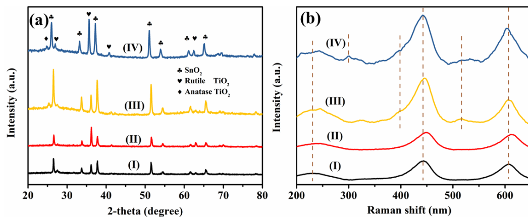
Figure 1. The XRD spectra (a) and the Raman patterns (b) of TNRs (I), H-TNRs (II), A-H-TNRs (III) and hybrid CAHT NRs (IV).
