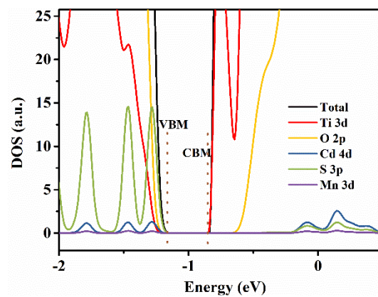
Figure S10. Partial electronic density of states for CAHT NRs hybrids.
