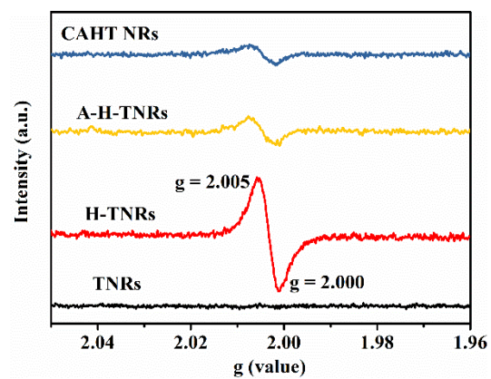
Figure S4. Typical EPR spectra of the as-prepared samples.
