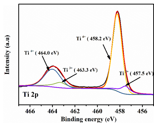
Figure S13. The XPS Ti 2p core-level spectrum of the H-TNRs film.
