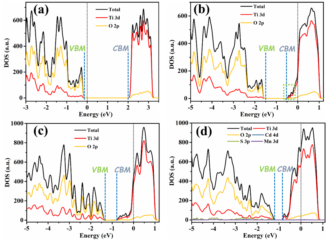
Figure 7. Total and partial electronic density of states (TDOS and PDOS) for TNRs (a), H-TNRs (b), A-H-TNRs (c) and CAHT NRs hybrids (d).
