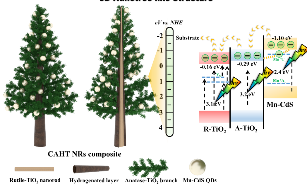
Scheme 2. The schematic and energy level alignment illustrating the as-proposed charge photogeneration and transfer mechanism in the CAHT NRs film enhanced PCP application.
