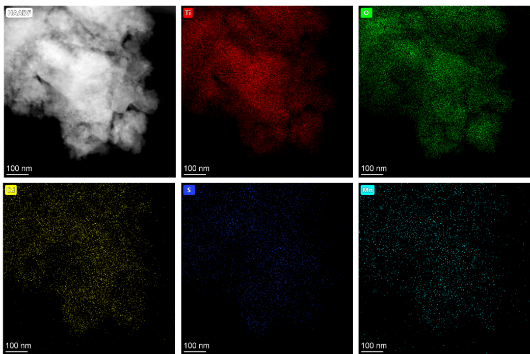
Figure S2. EDS element mapping images of Ti, O, Cd, S and Mn from the selected area of CAHT NRs composite.
