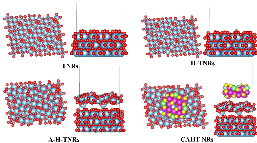
Figure S14. Space-filing structural models of as-prepared films from the top and side views. (Ti: blue, O: red, Cd: violet, S: yellow, Mn: green)
