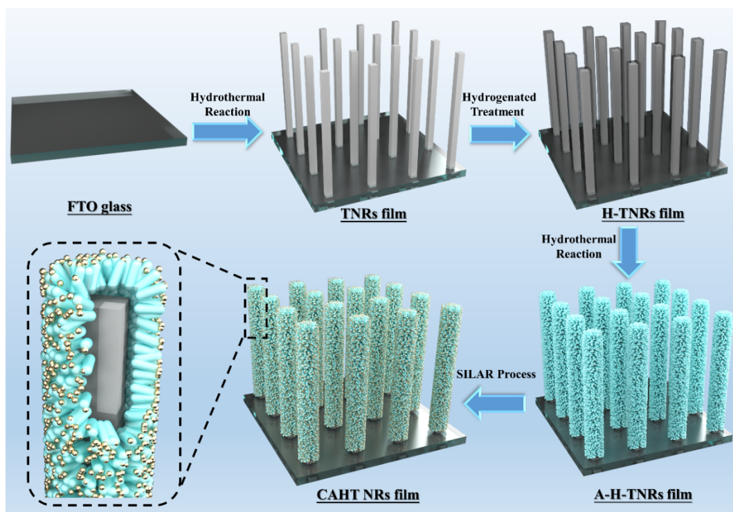
Scheme 1. Schematic illustration of the synthesis process for the quaternary CAHT NRs hybrid composite film.
