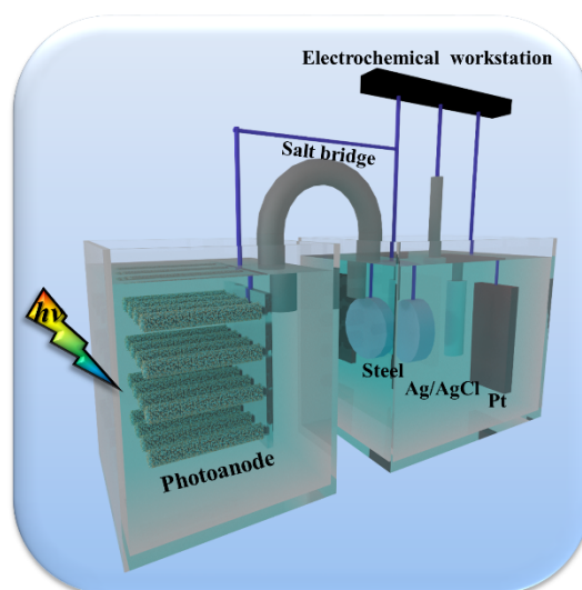
Figure S12. Schematic of the photoelectrochemical test configuration
