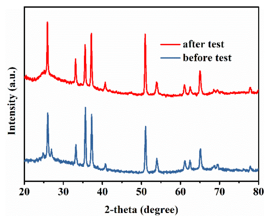
Figure S9. The XRD spectrum of the CAHT NRs hybrid composite film before and after 8 hours' PCP test.
