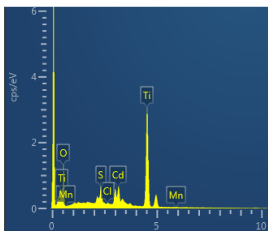
Figure S8. EDS spectrum of CAHT NRs after 8 hours' PCP test
