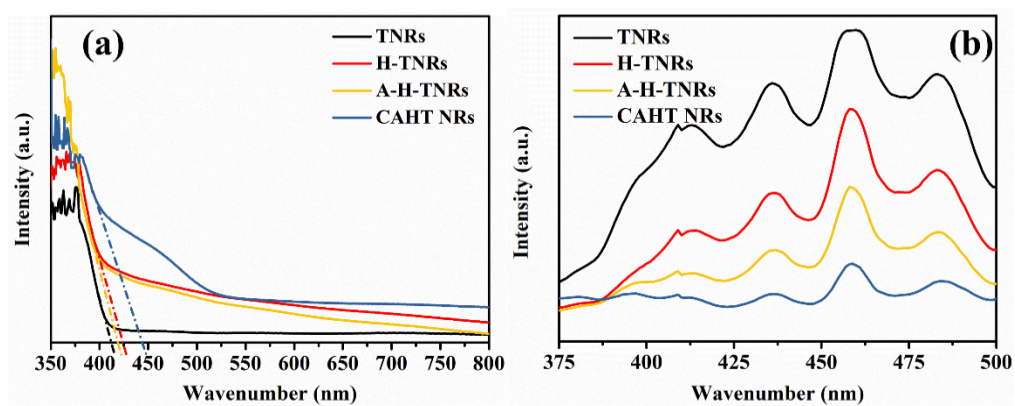
Figure S5. UV-visible diffuse reflectance spectra (a) and PL spectra (b) of quaternary CAHT NRs hybrid composite films.
