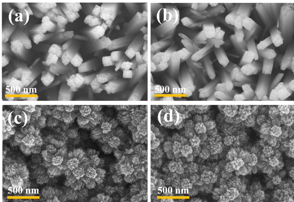
Figure 2. Top-view SEM images of the TNRs (a), H-TNRs (b), A-H-TNRs (c) and CAHT NRs (d) composite films.
