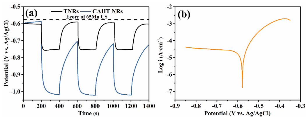
Figure S6. The potential variations (a) between the as-prepared samples in 0.1 M Na_2S and 0.2 M NaOH mixed solution and 65Mn CS electrode in 3.5 wt% NaCl solution under intermittent simulated solar light irradiation; The polarization curves (b) of uncoupled 65Mn CS electrode in 3.5 wt% NaCl solution.
