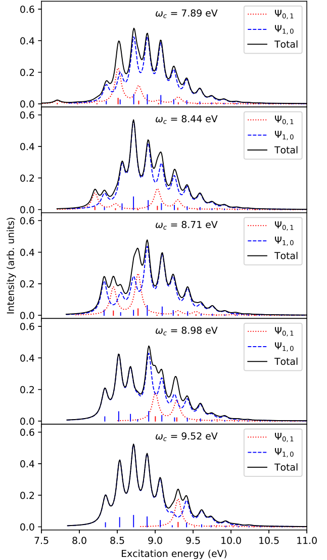
FIG. 11: Vibrationally-resolved spectra for CO using \gamma = 0.1 with coupling turned off, compared to the fully electronic A^1\Pi state spectrum
