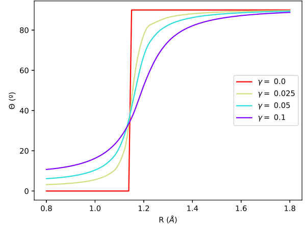
FIG. 6: CO mixing angle ( \theta , ^\circ ) as a function of the internuclear distance ( R , \text{\AA} ) calculated from the wavefunction coefficients
