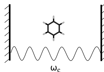
FIG. 1: Schematic representation of a molecule in an optical cavity
