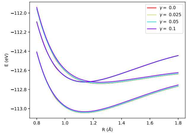
FIG. 7: Diabatic energy curves for CO using \omega_c = 8.7 eV and for different values of \gamma
