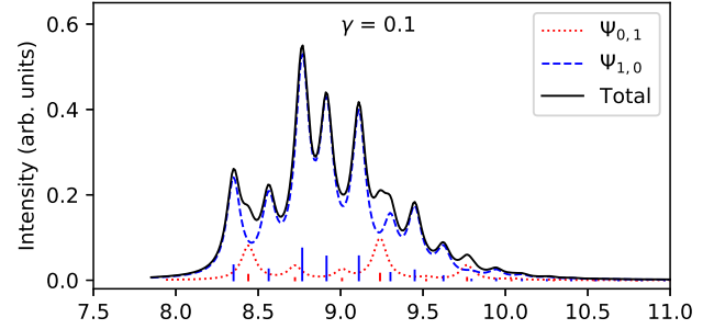
FIG. 9: Vibrationally-resolved spectra for CO using \omega_c = 8.7 eV and \gamma = 0.1 , using the diabatic states calculated in the adiabatic basis
