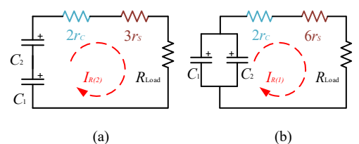
Fig. 7 Equivalent circuit of the load current path considering the parasitic parameters: (a) at +2 level; (b) at +1 level.
