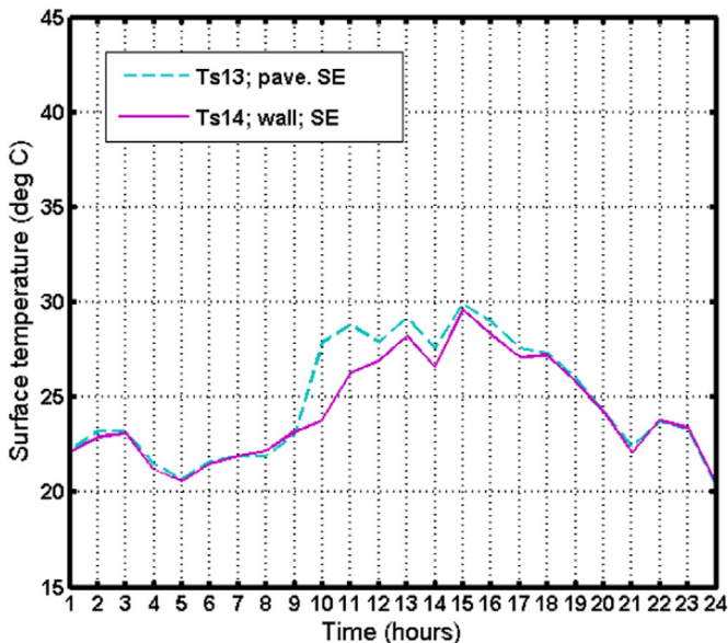
Fig. 8. Evolution of surface temperatures at the Borough Road (WS6) on 21 July 2010.
