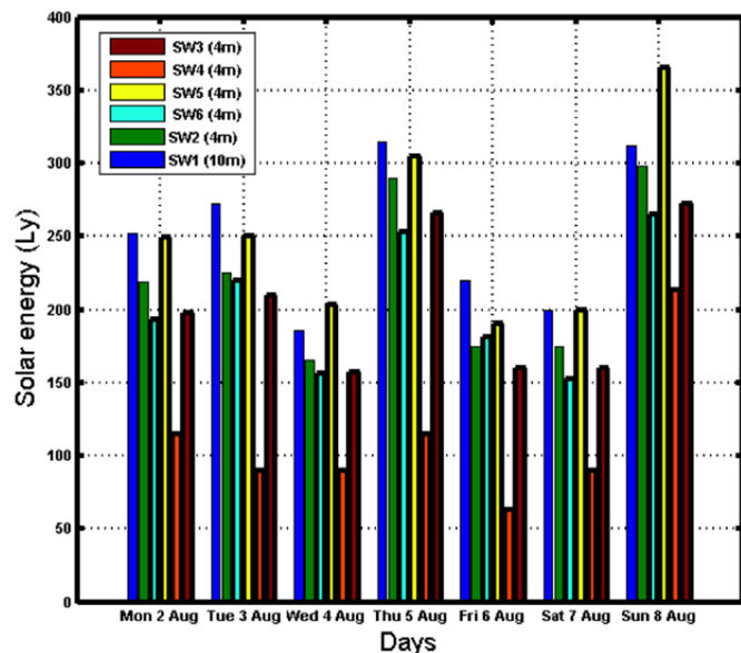
Fig. 10. Daily solar energy distribution at London site, from 2 to 8 August 2010.
