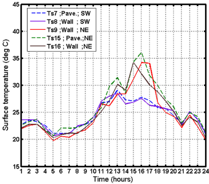
Fig. 7. Evolution of surface temperatures at the Keyworth Street (WS4), on 21 July 2010.
