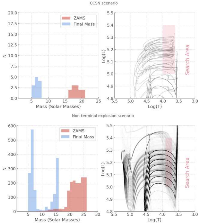
Figure 13. Mass distributions (ZAMS and final) and evolutionary tracks of BPASS models matching the L and T derived from DUSTY modelling. The upper (lower) panel shows the CCSN (non-terminal) scenario. Each evolutionary track is plotted at a low transparency and therefore the lighter the tracks, the rarer they are in our matches. We mark the search area in T and L from Section 2 in each HR diagram.
