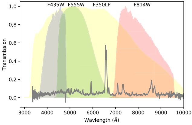
Figure 3. HST filters used for the pre-explosion light curve, compared with the +271 d spectrum. Only F350LP covers the strong H\alpha emission seen at this epoch.
