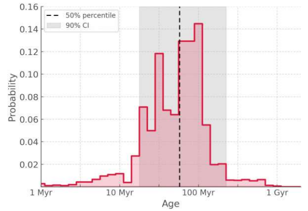
Figure 8. Probability distribution of the age of the 150-pc stellar neighbourhood of AT 2016jbu found using AGEWIZARD. The 90 per cent confidence interval is highlighted in grey.
