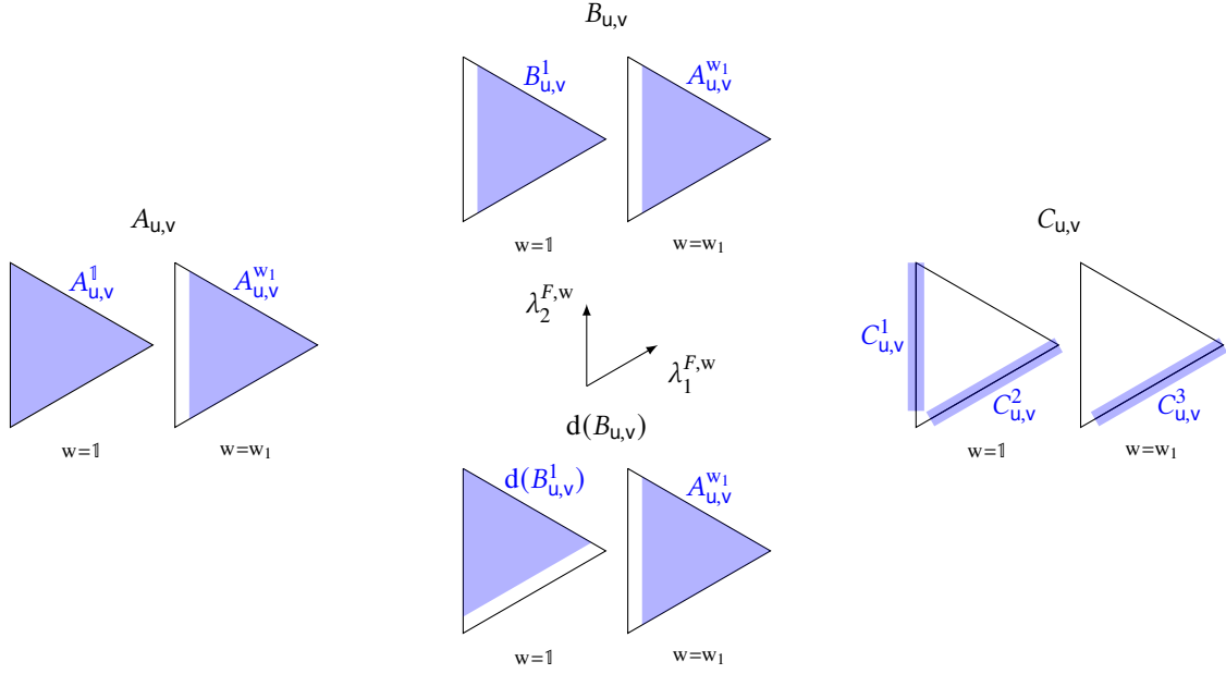
FIGURE 3. The fractional parts \widehat{\lambda}^{F,w} \in \widehat{\mathcal{P}}_{\geq}^{v-1} of the admissible weights, projected onto the real slice of \mathfrak{h}^* , that define highest-weight A_2(u,v) -modules (left), semirelaxed highest-weight A_2(u,v) -modules for the parabolic \mathfrak{p} (centre top) and d(\mathfrak{p}) (centre bottom), and relaxed highest-weight A_2(u,v) -modules (right).
