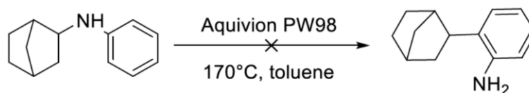
Scheme 1. Hofmann-Martius rearrangement of A to B.
