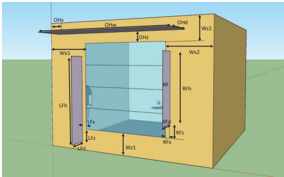
Figure 8.8 Parametric office geometry with variables for robust design test. Note that the window is modeled as four windows for the purpose of simulating partially closed shades.
