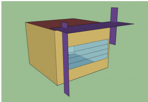
Figure 8.10 Optimal fixed shading design corresponding to the lowest predicted lighting energy use.
