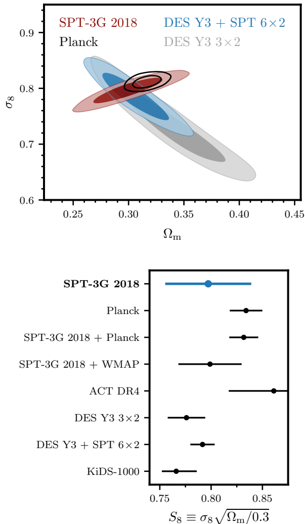
FIG. 11. Top panel: Constraints in the \sigma_8 vs. \Omega_m plane from SPT-3G 2018 (red), Planck (black line), a joint analysis of DES Y3 galaxy position and lensing data and SPT and Planck CMB lensing data ( 6 \times 2 , blue) [54], and DES Y3 joint galaxy density and weak lensing data ( 3 \times 2 , gray) [52]. The combined structure growth parameter, S_8 \equiv \sigma_8 \sqrt{\Omega_m/0.3} , varies perpendicular to the degeneracy direction of the DES data.
