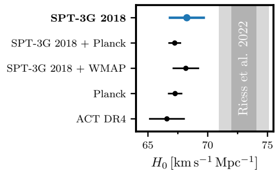
FIG. 10. Compilation of H_0 constraints from combinations of different CMB data sets assuming \Lambda CDM: SPT-3G 2018, Planck [1], WMAP [15], ACT DR4 [5]. The vertical gray band indicates the 2 \sigma constraint from the most precise supernovae and distance ladder analysis [47]. SPT-3G 2018 data allow for a precision constraint on H_0 effectively independent from Planck data that deepens the Hubble tension.
