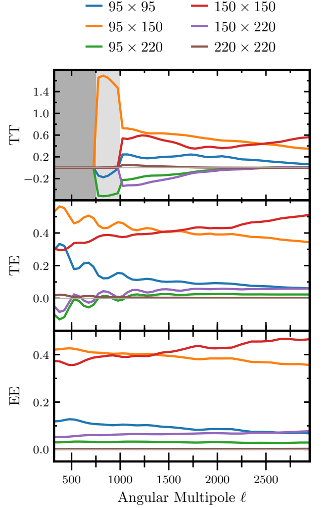
FIG. 6. Relative weight of each multifrequency spectrum entering the minimum-variance combination (diagonal elements of the mixing matrix). The gray shaded areas indicate the different \ell_{\min} cuts of the TT spectra. Overall, the 95 \times 150 GHz and 150 \times 150 GHz spectra contribute the most weight. For TT data, all spectra bar the 220 \times 220 GHz band powers are non-negligible at intermediate \ell and the 95 \times 95 GHz TE data are important on large angular scales.
