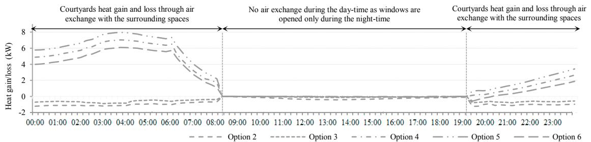
Fig.5. Average heat gain and loss in (KW) in the courtyards resulted from the air exchange with the surrounding spaces
