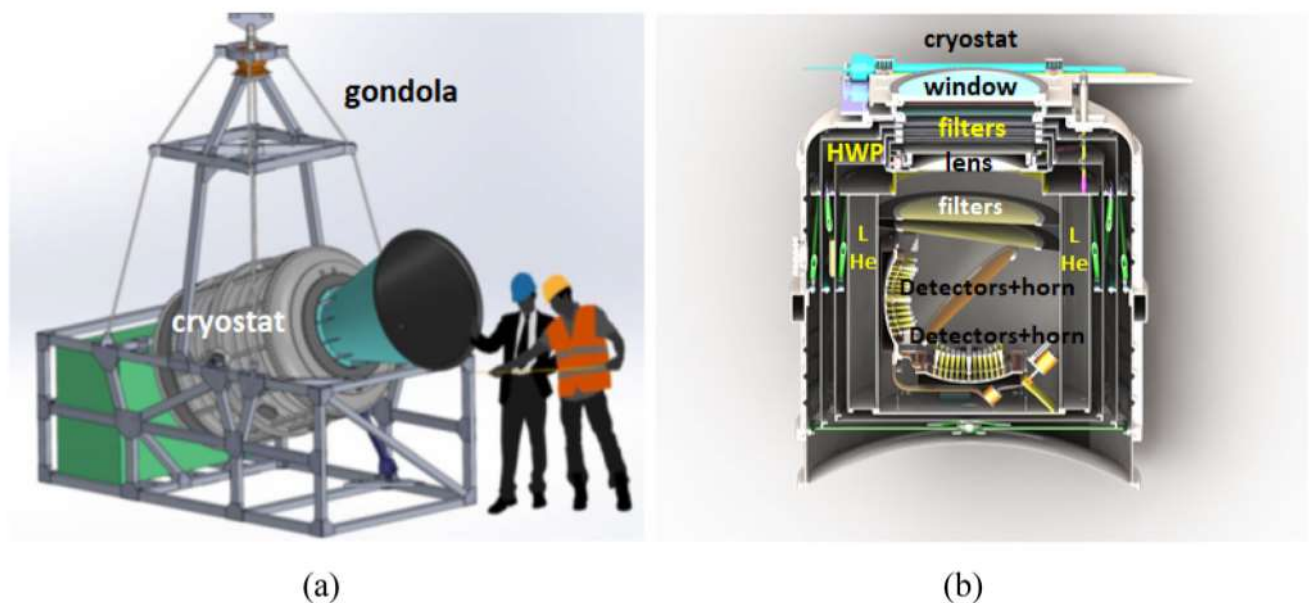
Fig. 3 a sketch of the SWIPE gondola and of the cryostat. b sketch of the inner part of the cryostat
