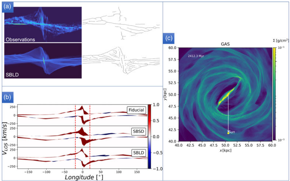
Figure 1. A) Left: l - v maps of the observations (top) and the best model at its optimal time/viewing angle. Right: the respective extracted skeletons. The ranges of these l - v are: |V_{LOS}| \pm 280 km/s and |l| \pm 60^{\circ} . B) Terminal velocity comparison of the Dame et al. (2001) CO observations with our three different models (as labelled). Vertical dashed red lines delimit the inner and outer Galaxy regions ( |l| < 20^{\circ} ). Red regions denote areas covered by the observations and not the models, and blue regions the reverse. C) Top-down view of the surface density of the gas of our best fit model (SBLD at a time \sim 2.4 Gyrs) with the Sun at 270^{\circ} .
