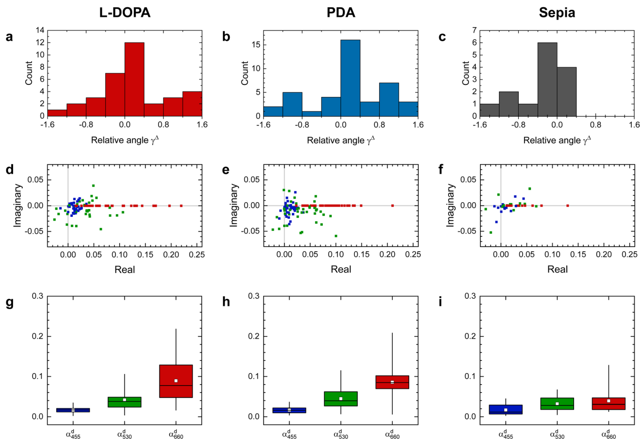
Fig. 4 (a–c) Histograms of \gamma^\lambda , the relative angle of the change of dichroism from 455 nm to 530 nm and 455 nm to 660 nm, for the L-DOPA (a), PDA (b), and sepia (c) NPs. (d–f) Dichroism in complex representation Z_\lambda^d \exp(-i\gamma^\lambda) , at 455 nm (blue), 530 nm (green), and 660 nm (red) for the L-DOPA (d), PDA (e), and sepia (f) NPs. (g–i) The distribution of \alpha_\lambda^d at each wavelength for L-DOPA (g), PDA (h), and sepia (i) NPs. The coloured boxes represent the interquartile range, with the horizontal line representing the median, and the white squares the mean. The vertical lines extend between minimum and maximum.
