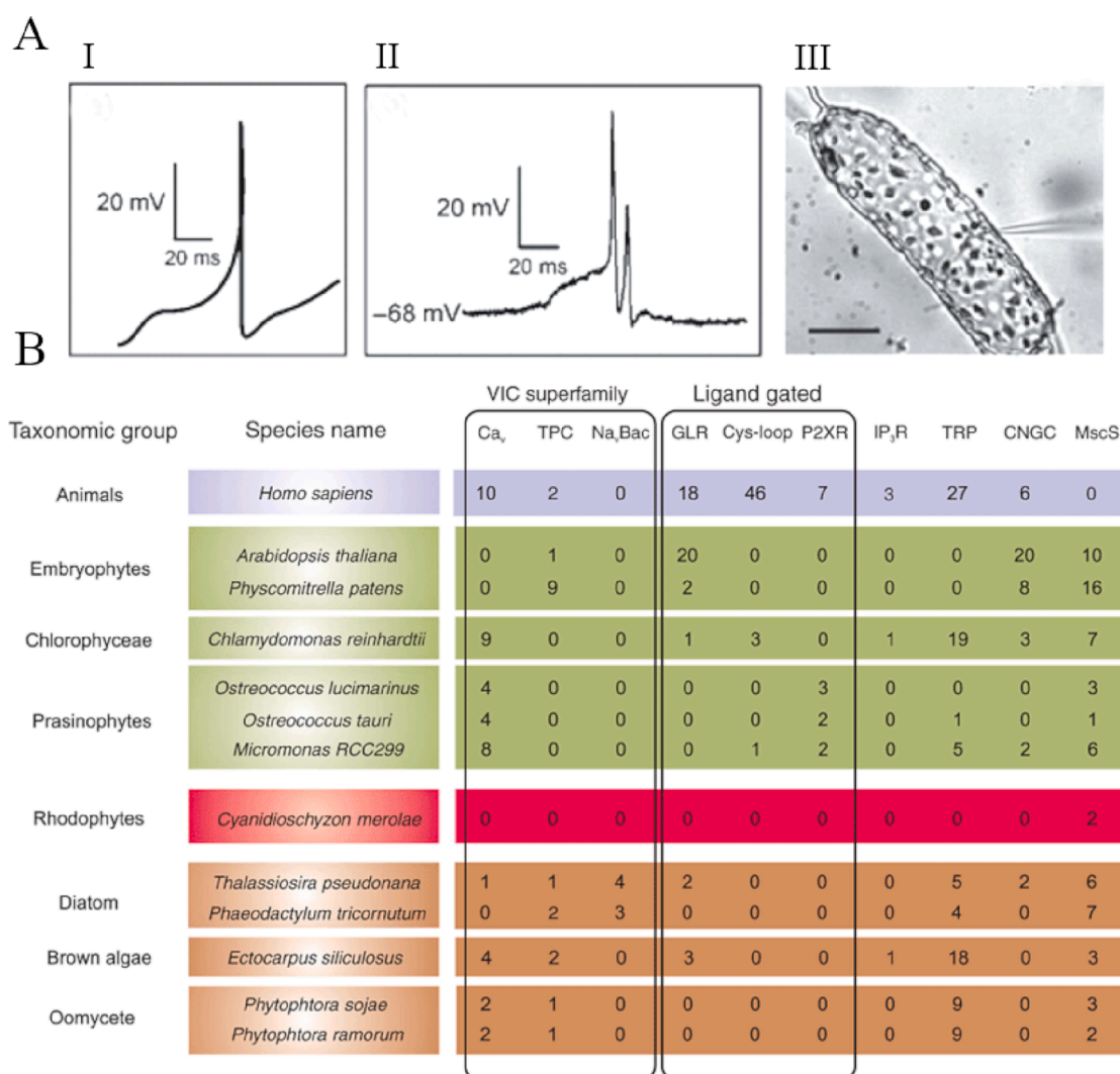
Fig. 2. Electroactive microalgae (A) Action potentials in squid and in diatom species. (I) Representative example of an action potential recorded from the giant squid. Reproduced with permission from [42] and [37], copyright Wiley & Sons; (II) A spontaneous action potential recorded in the diatom Odontella sinensis . Reproduced from [20] Copyright PLOS under CC BY 4.0 license ( https://creativecommons.org/licenses/by/4.0/ ); (III) A single cell of O. sinensis with intracellular recording electrode in place. Scale bar represents 20 \mu\text{m} . Reproduced from [24] copyright PLOS under CC BY 4.0 licence ( https://creativecommons.org/licenses/by/4.0/ ). (B) Distribution of the major classes of \text{Ca}^{2+} -permeable channels identified in photosynthetic eukaryote genomes. Ca v , voltage-dependent \text{Ca}^{2+} channel; CNGC, cyclic nucleotide-gated channel; Cys-loop, cysteine loop; GLR, glutamate receptor; IP 3 R, inositol-1,4,5-trisphosphate receptor; MscS, mechanosensitive ion channel; Na 2 Bac, single-domain, bacterial-type channel; P2XR, purinergic P2X receptor; TPC, two-pore \text{Ca}^{2+} channel; TRP, transient receptor potential; VIC, voltage-gated ion channel. Reproduced with permission from [42], copyright Wiley & Sons.
