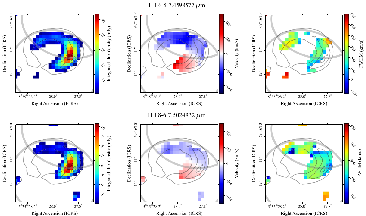
Figure 7. Same as Figure 6 but for a selection of HI lines.
