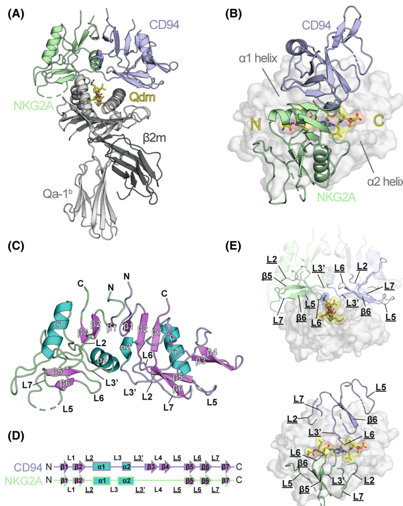
Fig. 1. Structure of murine CD94–NKG2A bound to Qdm presented by Qa-1 b . (A) Structural overview of mCD94–NKG2A in complex with the Qdm peptide (AMAPRTLTL) presented by Qa-1 b . CD94, NKG2A, Qa-1 b and \beta 2m represented as cartoon and coloured by chain; Qdm peptide = sticks, coloured by atom (carbon = yellow, oxygen = red, nitrogen = blue). (B) Birdseye view of mCD94–NKG2A binding atop the Qa-1 b peptide binding groove. mCD94–NKG2A represented as cartoon with Qa-1 b shown as a surface representation with MHC \alpha 1 and MHC \alpha 2 helices shown as cartoon representation. Qdm is shown as both sticks and surface and coloured by atom. (C) Cartoon representation of mCD94–NKG2A heterodimer domain architecture (N and C termini labelled N and C respectively). Structural elements annotated according to secondary structure; \alpha -helices ([ \alpha ] teal), \beta -strands ([ \beta ] magenta) and loops ([L], CD94 blue, NKG2A green). (D) Schematic representation of mCD94–NKG2A heterodimer domain architecture. Arrows = \beta -strands, rectangles = \alpha -helices. Structural elements involved in ligand binding are underlined. (E) Arrangement of mCD94 and mNKG2A chains over Qa-1 b (surface, \alpha 1 and \alpha 2 helices = cartoon) and Qdm peptide (surface and sticks) from side (top) and birds-eye (bottom) views. Each binding structural element is rendered opaque and non-binding elements semi-transparent. mCD94 is located over the Qa-1 b \alpha 1 domain and Qdm P8 residue whilst NKG2A binds over the \alpha 2 domain and Qdm N-terminus resulting in a near perpendicular binding mode. Structural figures produced in PYMOL [49].
