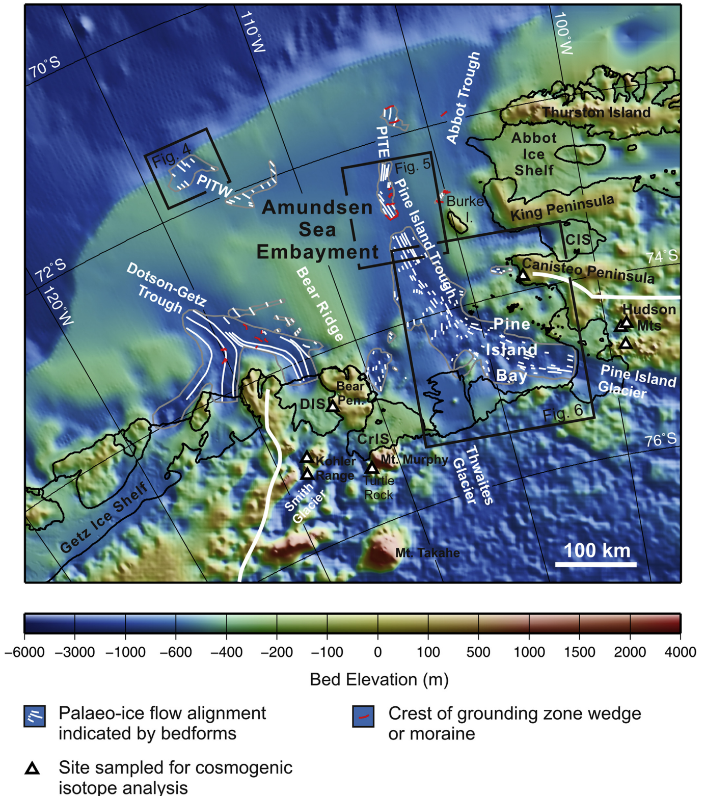
Fig. 3. Map of the Amundsen Sea Embayment showing main geomorphological features on the continental shelf and cosmogenic surface exposure age sample locations onshore, overlaid on Bedmap2 ice sheet bed and bathymetry (Fretwell et al., 2013), which is displayed with shaded-relief illumination from the upper right. Grey outlines mark areas in which bedforms indicative of past ice flow direction are observed in multibeam swath bathymetry data. Thin white lines indicate flow alignment. Red lines mark the crests of grounding zone wedges and moraines that represent past grounding line positions. Thick white lines mark major ice divides. Black rectangles outline areas shown in greater detail in Figs. 4–6. CIS – Cosgrove Ice Shelf; CrIS – Crosson Ice Shelf; DIS – Dotson Ice Shelf; PITE – Pine Island Trough East; PITW – Pine Island Trough West.
