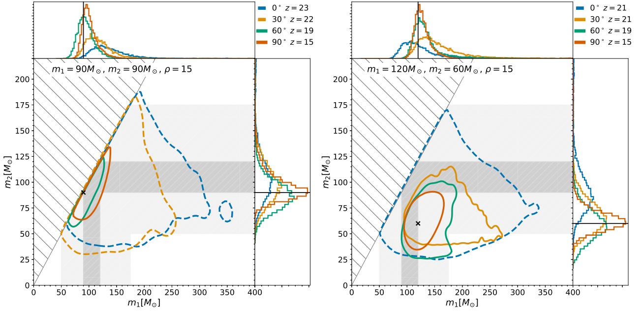
Figure B1. Inferred posteriors of component masses for binaries of total mass of 180 M_{\odot} which straddle, or sit within the upper mass gap. Results are shown for inclinations of \iota = 0^{\circ}, 30^{\circ}, 60^{\circ} , and 90^{\circ} , with the redshift of the system varied, as indicated in the labels, so that the signals are all simulated with an SNR of 15 in the ET–CE network, at the most sensitive sky location for the network. The grey region denotes the mass gap, whose location varies with the ^{12}\text{C}(\alpha, \gamma)^{16}\text{O} reaction rate, and the darker grey denotes the forbidden strip (Farmer et al. 2020). Simulated values are denoted by a black cross and contours show the 90 per cent credible region. Left: Binary with masses just below the mass gap: m_1 = m_2 = 90 M_{\odot} . Right: Binary with masses that straddle the mass gap: m_1 = 120 M_{\odot} and m_2 = 60 M_{\odot} .
