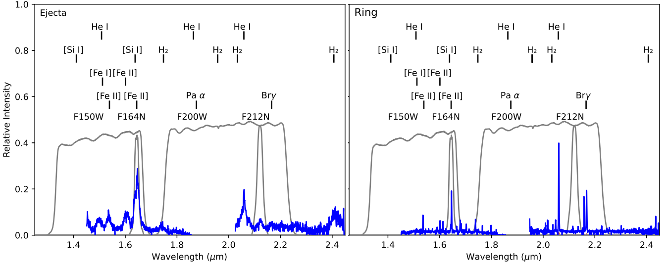
Figure 3. The filter transmission curves of the NIRcam short wavelength channel (grey lines). SINFONI spectra of the ejecta ( left ) and ring ( right ) in H - and K -bands (Larsson et al. 2016) are also plotted in blue lines, with line-identifications labelled.
