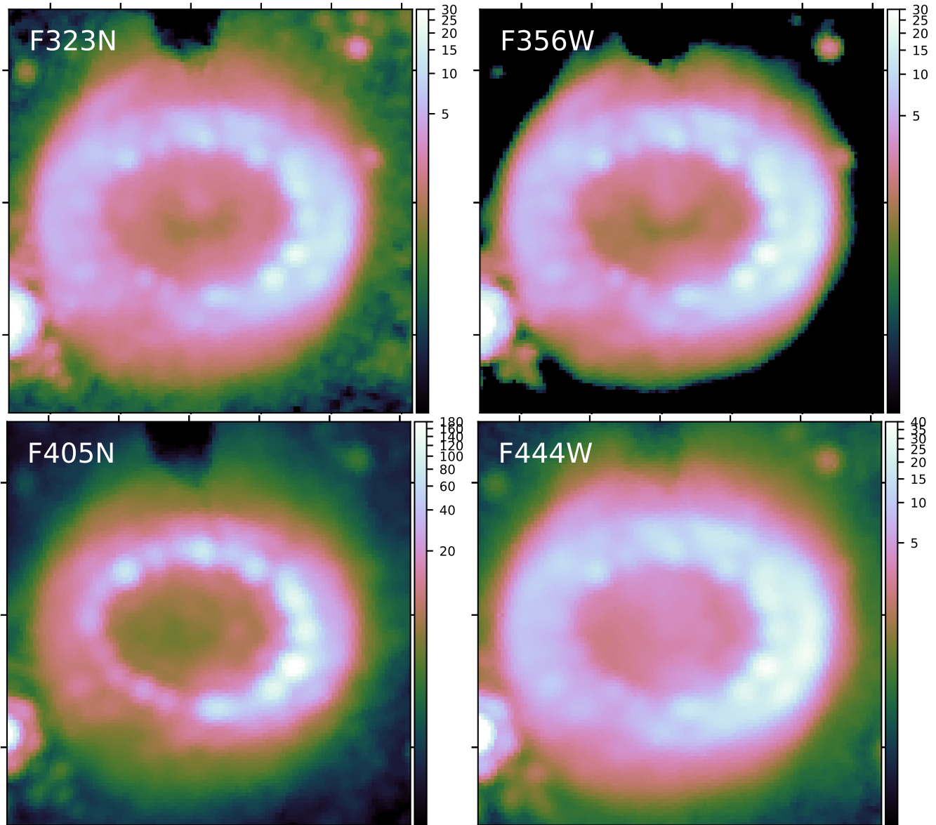
Figure 5. NIRCaw LW channel images. The outer spots exterior to the equatorial ring are as bright as the hot spots within the ring in the LW images, apart from F405N. The ejecta emission in the LW images is dominated by continuum, mostly due to dust. The dip in the centre of F323N, F356W and F405N is caused by dust self-absorption. Only two blobs are detected in these images. The F405N image traces both the dust continuum and Br \alpha in the ejecta. The coverage of the images is 3'' \times 3'' , with the north at the top, and the colour stretch is in the unit of MJy sr ^{-1} .
