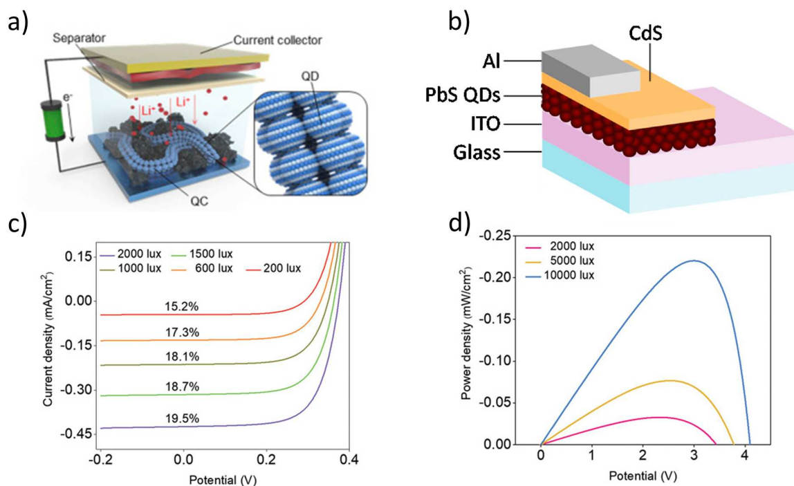
Fig. 12 a) Schematic structure of a CQD quantum chain incorporated into Lithium-ion battery. 139 b) Structure of a typical CQD solar cell. 140 c) J-V Curves at different indoor irradiances and their respective PCE values and d) Power Density - V curves at different irradiances for a PbS based photovoltaic cell. 141
