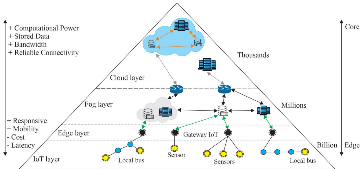
Fig. 5 Showing the different layers of the network, starting from the central cloud layer out into the edge and IoT layers. PERMISSION 57
