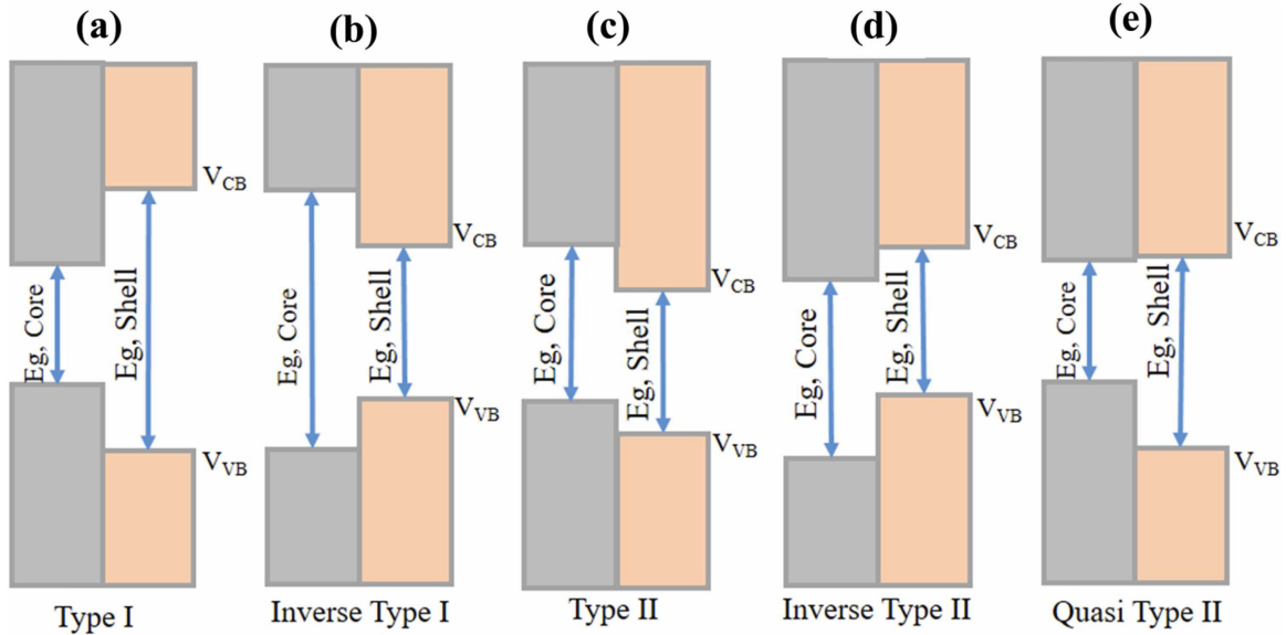
Fig. 3 Different types of core-shell structured QDs classified based on their bandgaps and band alignments. 23
