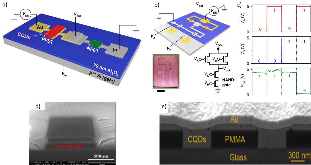
Fig. 14 a) The schematic structure of a CQD CMOS inverter, b) a schematic illustration (top), its picture (bottom left) and the circuit diagram (bottom right) of a NAND gate made from the p and n-type CQD FETs and c) the outcomes of the NAND gate for four different input configurations. 89 d) Cross-sectional SEM image of the H-SiN/CQDs/L-SiN waveguide. 157 e) Cross-sectional SEM image of a Y-splitter made from CQDs and PMMA 159
