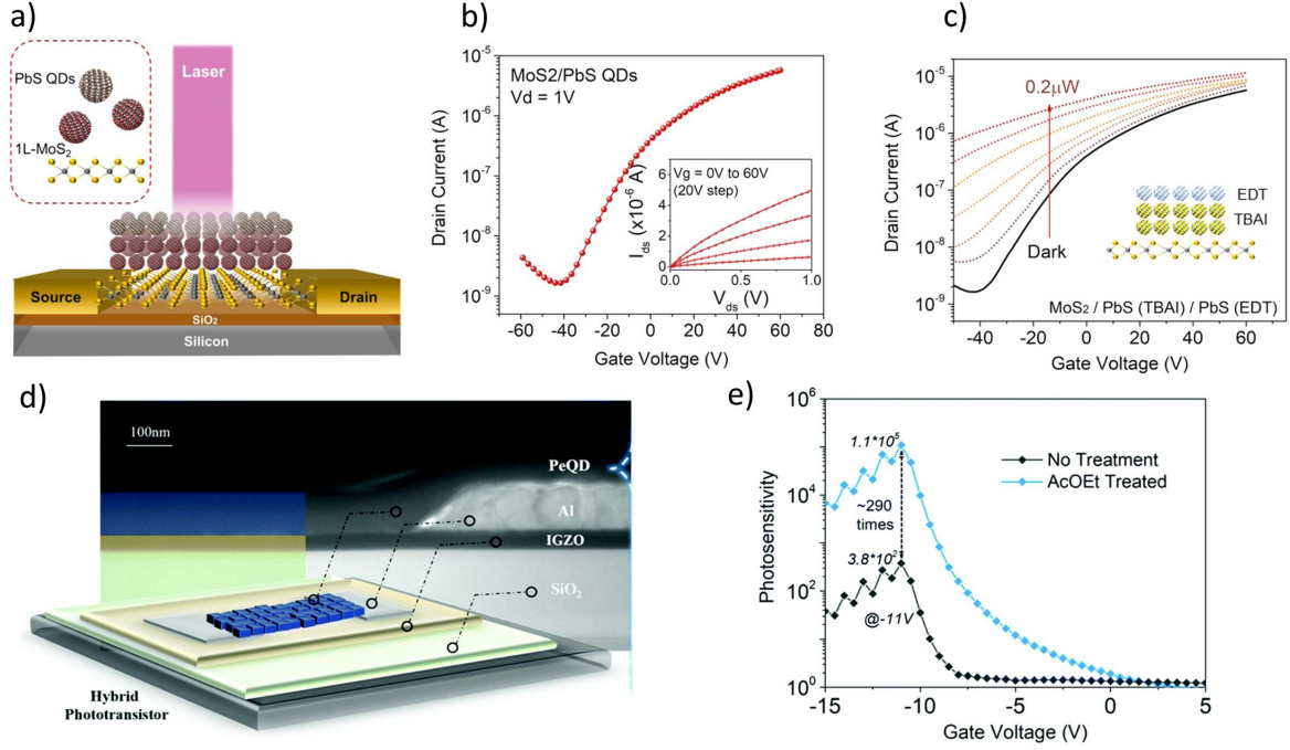
Fig. 9 a) The structure of a PbS/MoS 2 phototransistor, its respective b) I_D - V_G graph (inset: I_D - V_D for different V_G ) and c) I_D - V_G graph at different illumination powers. 94 d) The structure of hybrid perovskite QD and its e) PR - V_{GS} graph. 95
