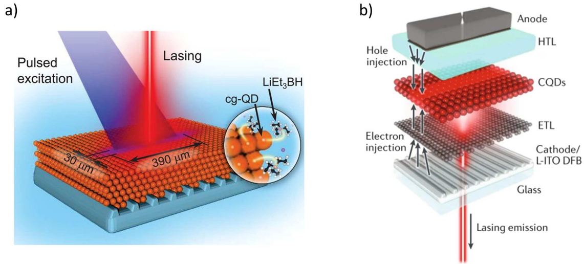
Fig. 15 Structure of a) an optically pumped CQD laser operating via a DFB structure 169 and b) a potential electrically pumped CQD laser, demonstrated to work by pumping optically 170
