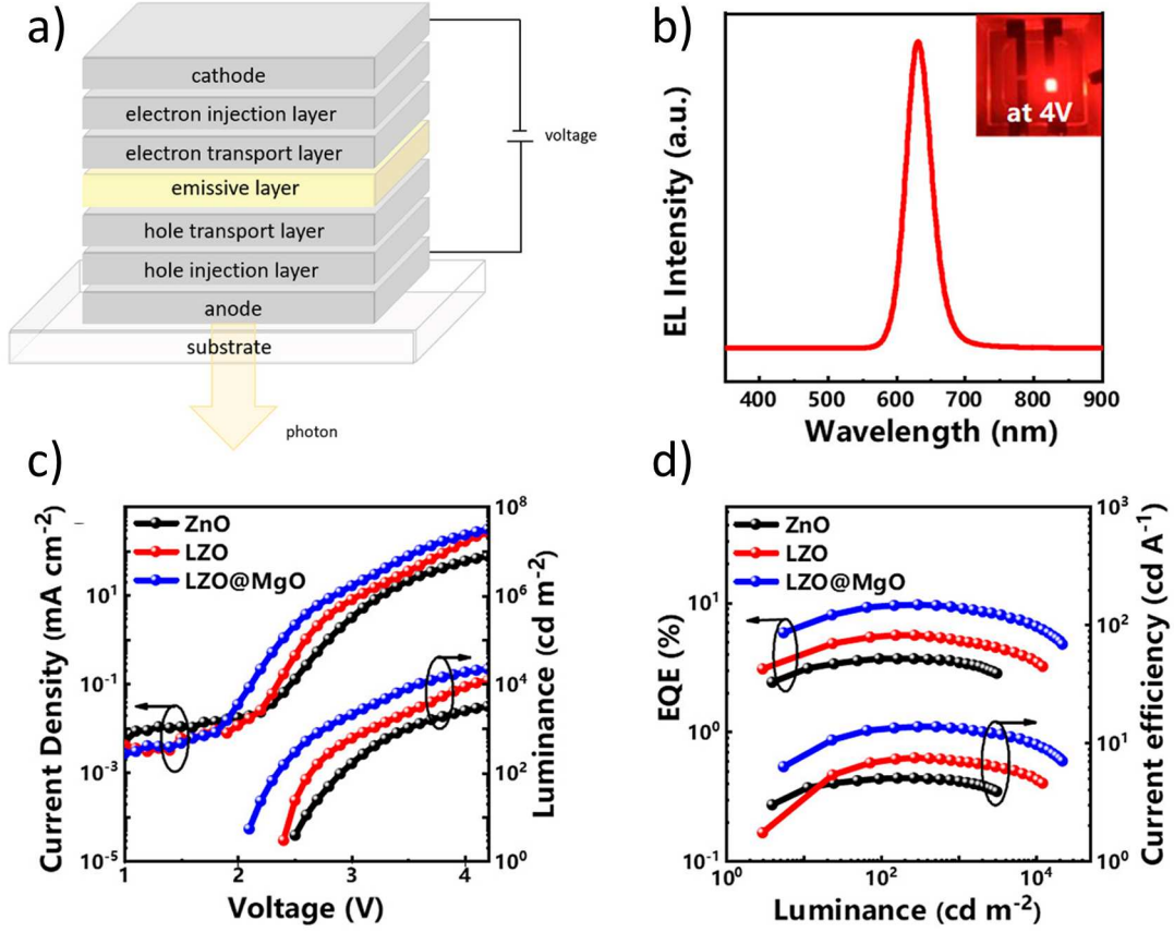
Fig. 10 a) The general structure of QLEDs. b) The EL spectra and the c) CD-V-L and d) EQE-L-CE graphs of an InP based QLED with different ETLs. 122
