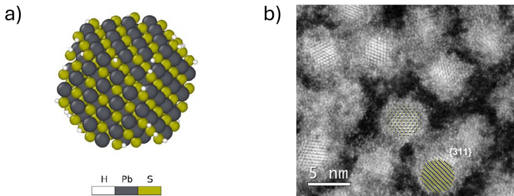
Fig. 1 a) Visualisation of a passivated sulfur-rich PbS QDs and b) High-resolution high-angle annular dark-field scanning transmission electron microscopy (HAADF-STEM) image of PbS QDs after cleaning with methanol. 3
