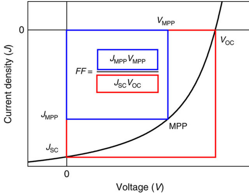
Fig. 13 Current Density - Voltage graph for a photovoltaic cell, showing the positions of important parameters 149
