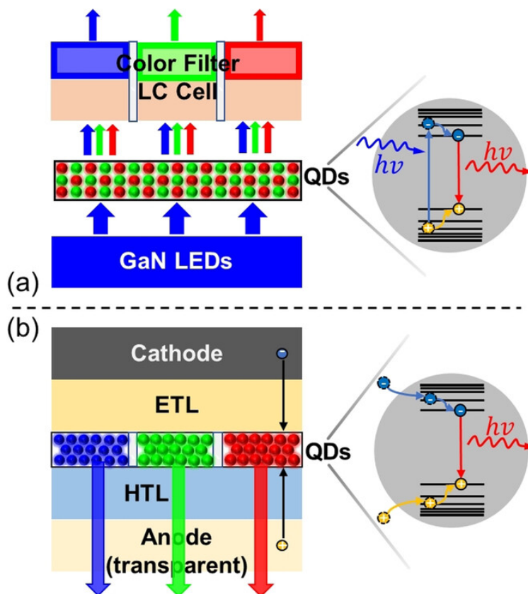
Fig. 11 a) The simplified structure of PL mode commercialised QLED TVs and their emission mechanism. b) Structure of EL mode QLEDs and their emission mechanism. PERMISSION 130
