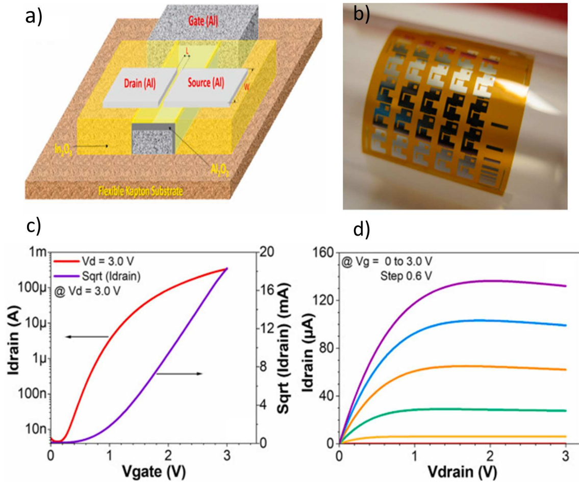
Fig. 7 a) The structure of an \text{In}_2\text{O}_3 flexible TFT on a flexible substrate. b) A camera image of the TFTs. The c) I_D - V_G and d) I_D - V_D graphs of the TFTs. 77
