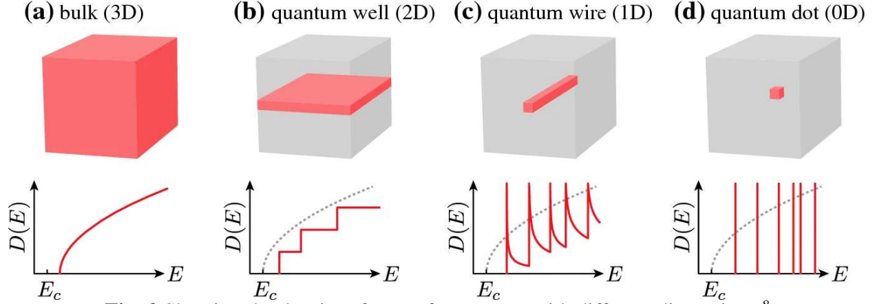
Fig. 2 Showing the density of states for systems with different dimensions. 8
