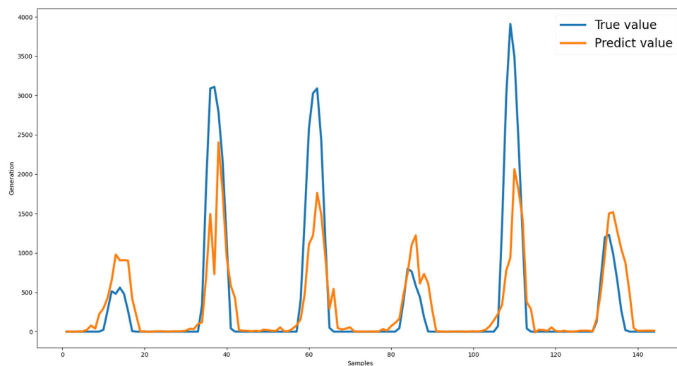
Figure 6: XGBoost PV generation prediction.
