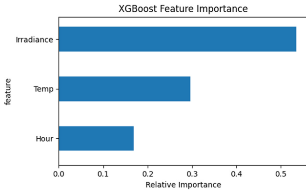
Figure 5: XGBoost time features analysis in PV generation data.
