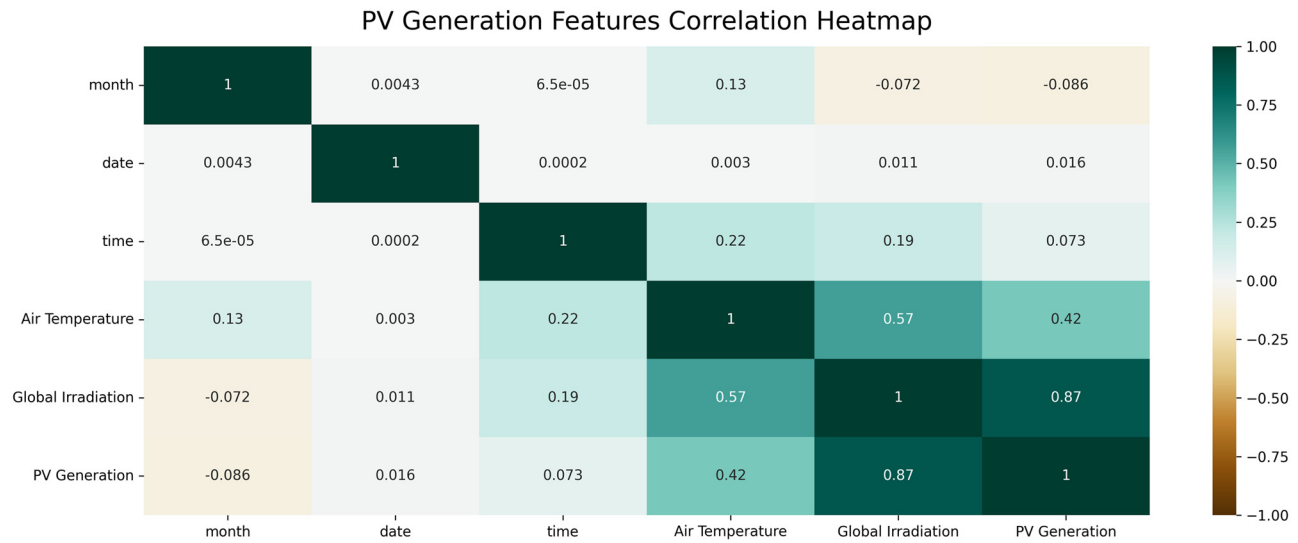
Figure 3: Heatmap of PV generation features correlation.
