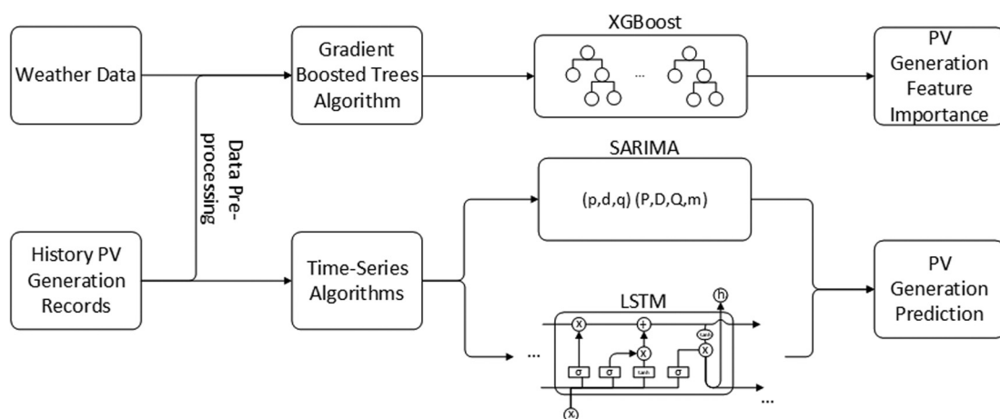
Figure 1: PV power generation prediction framework flowchart.
