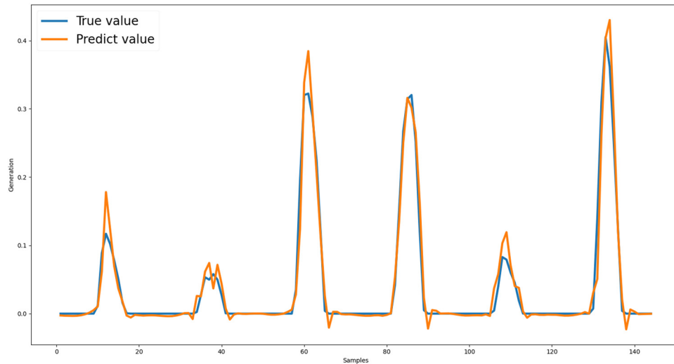
Figure 8: LSTM PV generation prediction.
