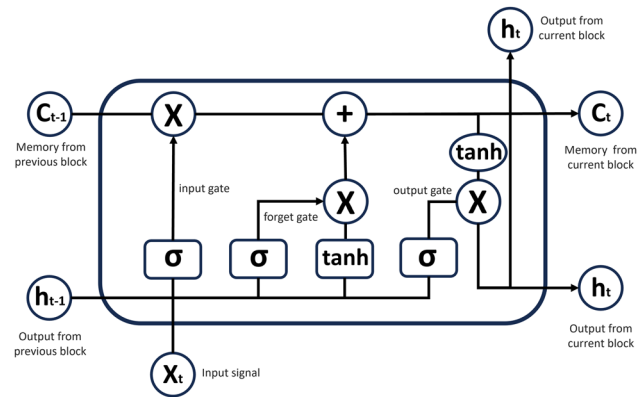
Figure 2: LSTM memory block demonstration.
