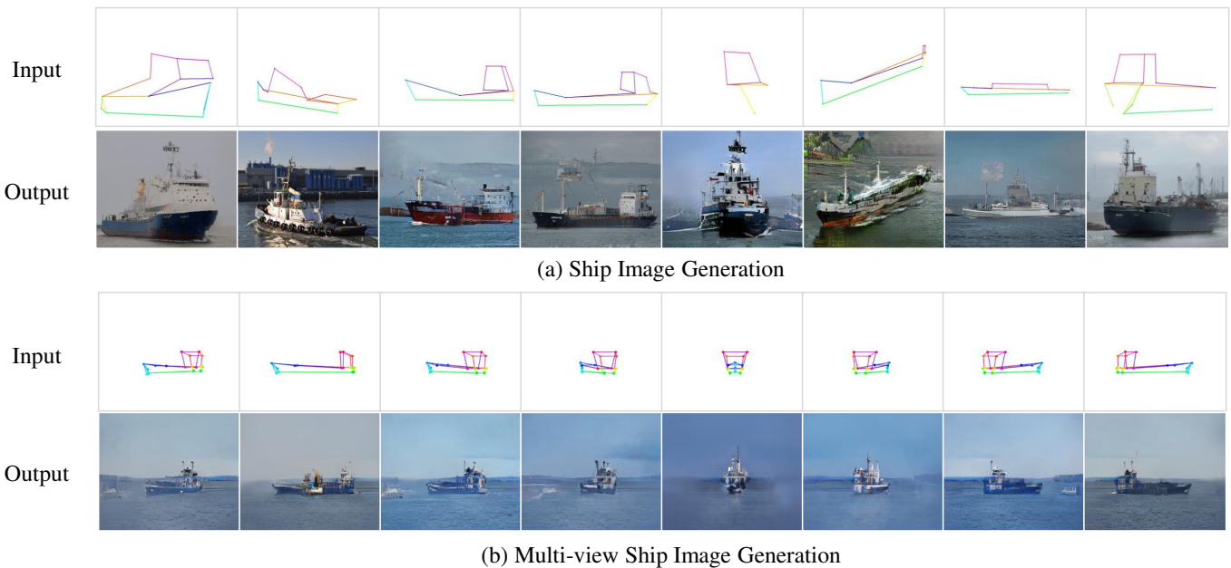
Fig. 13. Results for landmark-based ship image generation. (a) Ship image generation for different ships with corresponding ship skeletons. (b) Multi-view ship image generation for a single ship by rotating the 3D skeleton.
