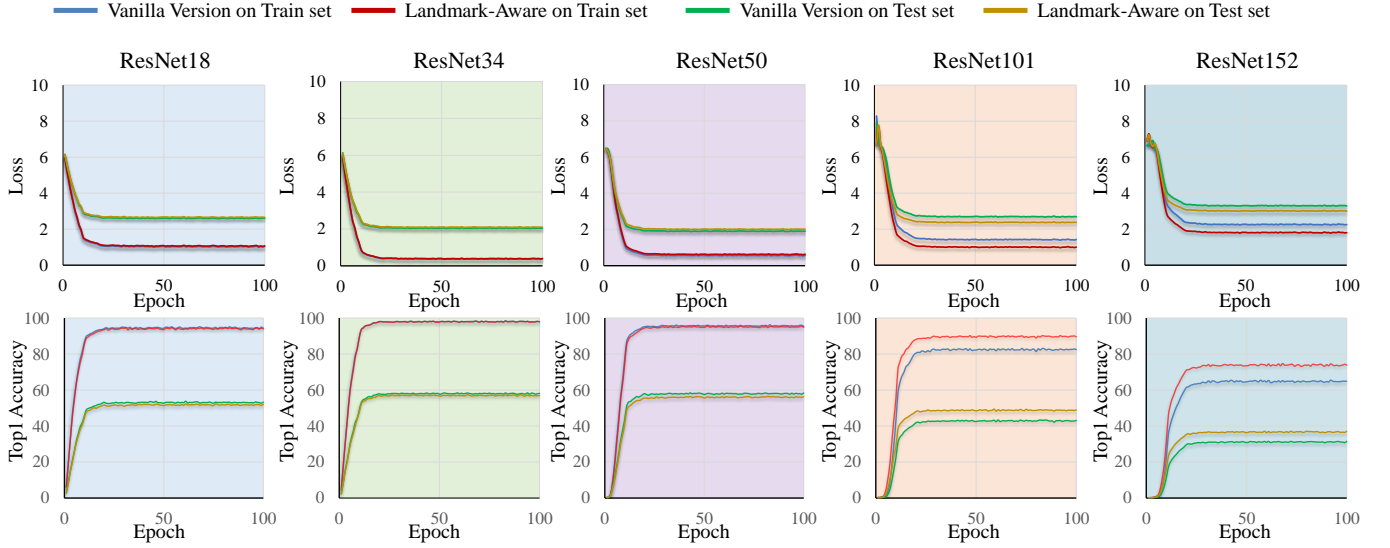
Fig. 12. Effect of landmark information on the performance of ship recognition. This figure shows the loss curves and average Top-1 performance of various methods with and without landmark information across 10 duplicate experiments.
