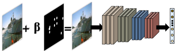
Fig. 11. Landmark-guided ship recognition. We replace the original input of the recognition model with a synthetic landmark-aware image where the regions around the landmarks are highlighted.
