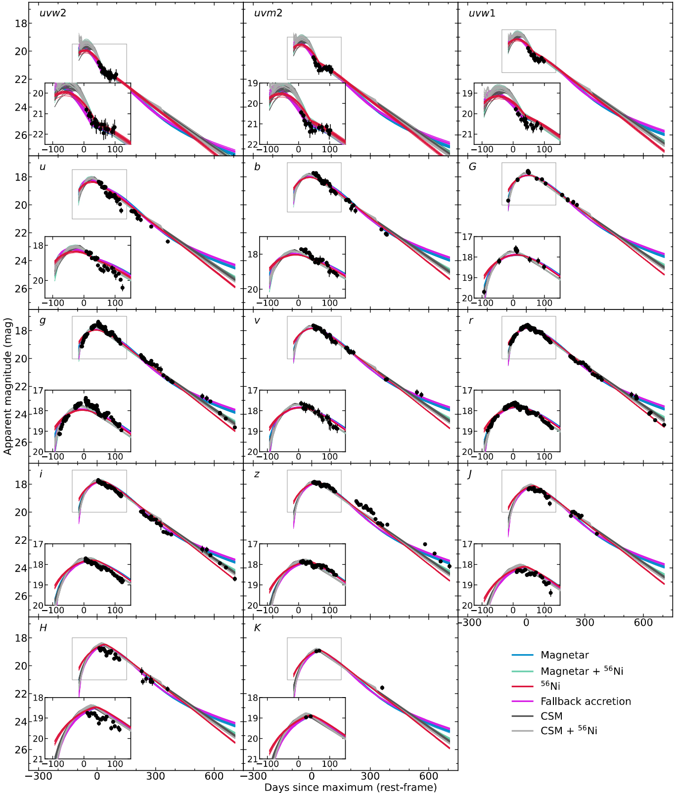
Fig. 24. Modelling of the light curves from the rest-frame UV to the NIR with MOSFiT. All models provide an adequate description of the data up to t_{\max}+400 days, though with differences in the fit quality. At later times, the models diverge. The pure nickel model is the only model that captures the evolution after t_{\max}+500 days and has physically meaningful parameters. The central engine models (magnetar and fallback) predict a flattening of the light curve due to a power-law-shaped heating rate in contrast to powering by ^{56}\text{Ni} that has an exponential energy deposition rate. The magnetar+nickel model also captures the full evolution. However, the inferred model parameters would be either physically implausible or require an exotic star, which we deem not viable. We note that the Keck photometry at t_{\max}+539 days and t_{\max}+562 days is not corrected for host contamination owing to the lack of Keck reference images to perform image subtraction. The expected host contribution is \approx 10\% .
