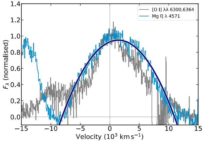
Fig. 17. [O I] \lambda\lambda 6300,6364 and Mg I] \lambda 4571 lines at t_{\max}+286.7 days. The Mg I] line is well fitted with a parabolic shape (dark blue), expected from an optically thick expanding shell (e.g. swept up CSM and unshocked SN ejecta), while the [O I] lines show a strong blue deficit because the line-forming region is still optically thick. The [O I] doublet is centred on the 6364 Å doublet component.
