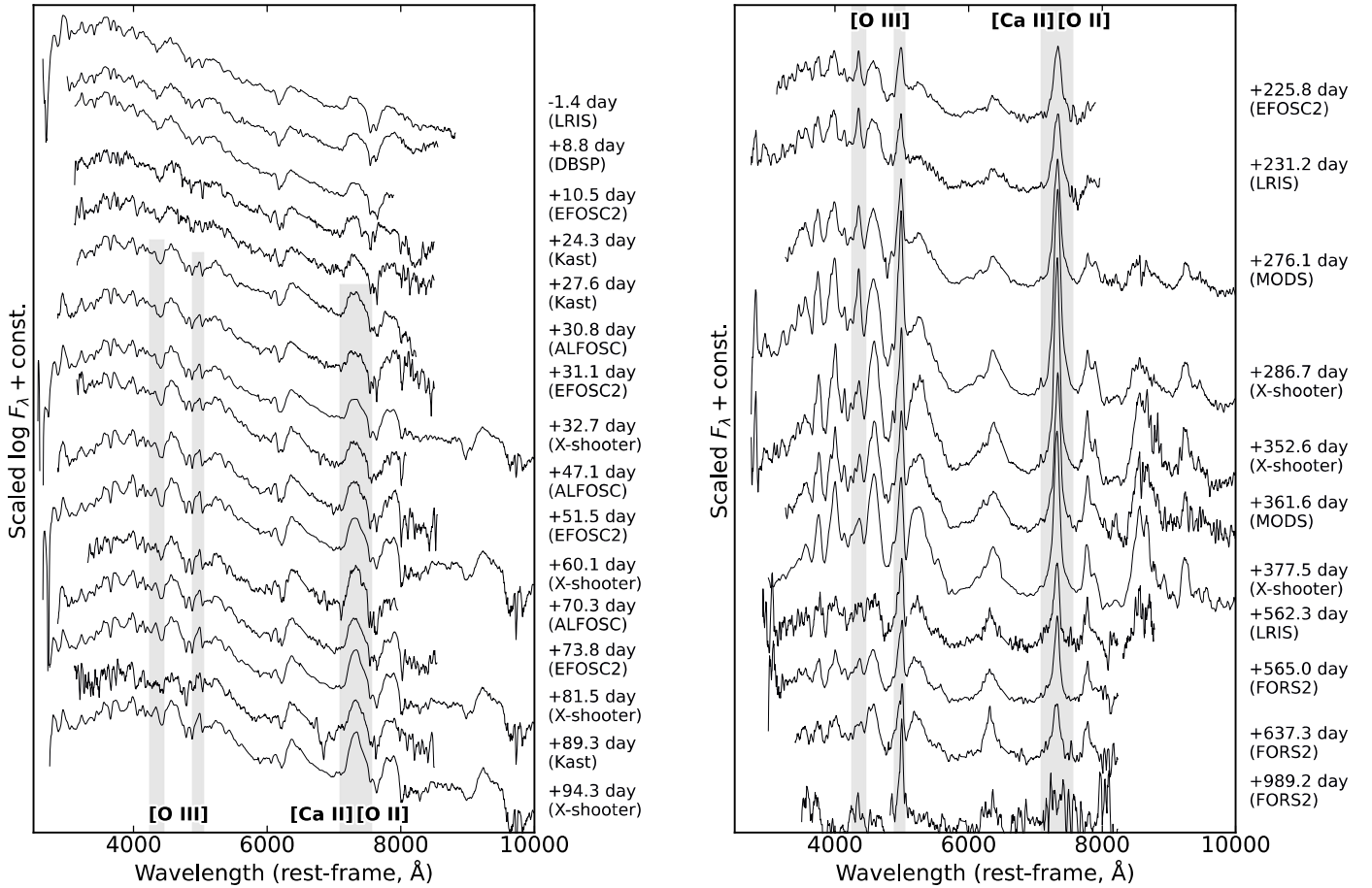
Fig. 6. Spectroscopic sequence from 2500 Å to 10 000 Å and from the time of maximum to t_{\max}+1000 days (rebinned to 5 Å and smoothed with a Savitzky–Golay filter). Spectra up to t_{\max}+100 days (left panel) are characterised by a blackbody continuum with superimposed absorption lines from the SN ejecta, expanding with a velocity of \sim 8500 km s ^{-1} . Between t_{\max}+100 and t_{\max}+225 days (while SN 2018ibb was behind the sun), the spectroscopic behaviour of SN 2018ibb evolved drastically. The late-time spectra (right panel) are characterised in the blue ( <5000 Å) by a pseudo-continuum and emission lines produced by the interaction of the SN ejecta with circumstellar material and in the red ( >5000 Å) by nebular emission lines from the ^{56}\text{Ni} -heated SN core. The regions with the fastest evolution are highlighted by the grey-shaded regions. Figure 7 shows the identification of the most prominent features of the photospheric and nebular phases. Regions affected by strong telluric absorption were clipped. Their locations are indicated in Fig. 7.
