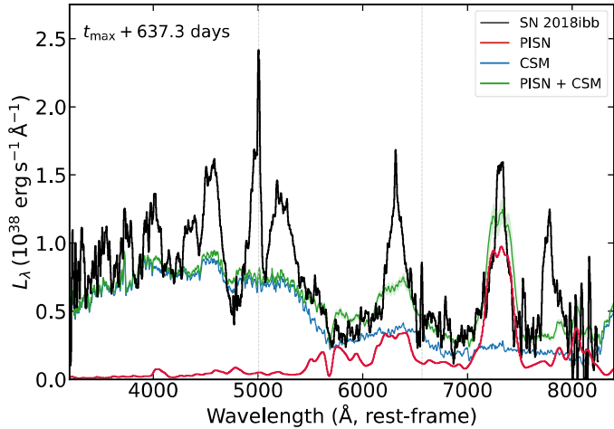
Fig. 27. Nebular spectrum of SN 2018ibb (black) at t_{\max}+637.3 days and its decomposition into a CSM interaction (blue) and PISN component (red). This decomposition reveals that the shape of the spectrum in the blue is similar to the pseudo-continuum seen in interaction-powered SNe (Type Ia-CSM, Ibn, Icn and IIn). The emission lines in the blue arise either from CSM interaction or from material in the CSM shell excited by the SN light. The dotted vertical lines indicate the location of strong galaxy emission lines.
