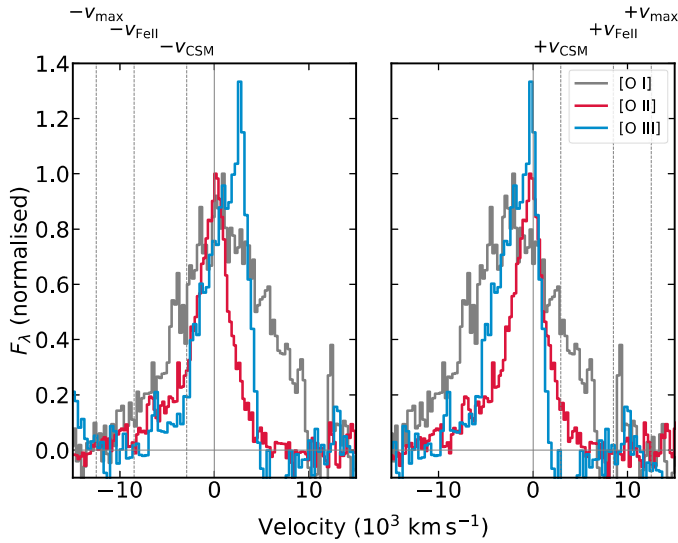
Fig. 19. [O I] \lambda\lambda 6300,6364, [O II] \lambda\lambda 7320,7330, and [O III] \lambda\lambda 4959,5007 line profiles at t_{\max}+565.0 days. The velocity scale is centred on the blue doublet component in the left panel and on the red component in the right panel. [O II] and [O III] only reach out to approximately the velocity of the CSM shell ( v_{\text{CSM}} ), much less than the photospheric velocity ( v_{\text{Fell}} ) and the maximum velocity of the ejecta ( v_{\text{max}} ). In contrast to that, the [O I] profile extends to \approx 12\,500\text{ km s}^{-1} . This points to [O II] and [O III] being produced close to the CSM shell whereas [O I] is produced in the SN ejecta.
