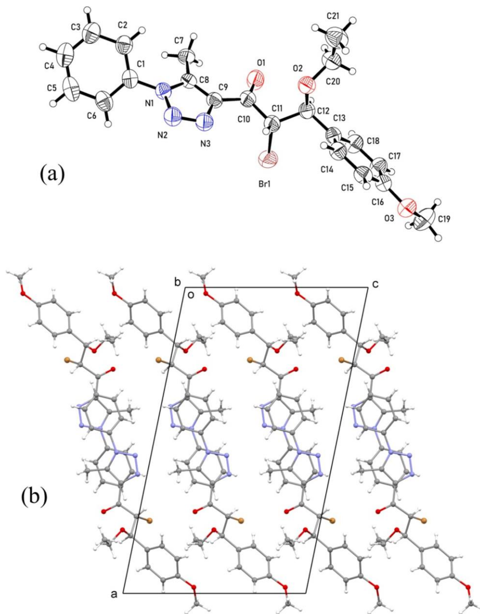
Fig. 3. (a) An ORTEP representation of 16 showing atomic displacement ellipsoids at 50 % probability and (b) crystal packing viewed down the b axis.
