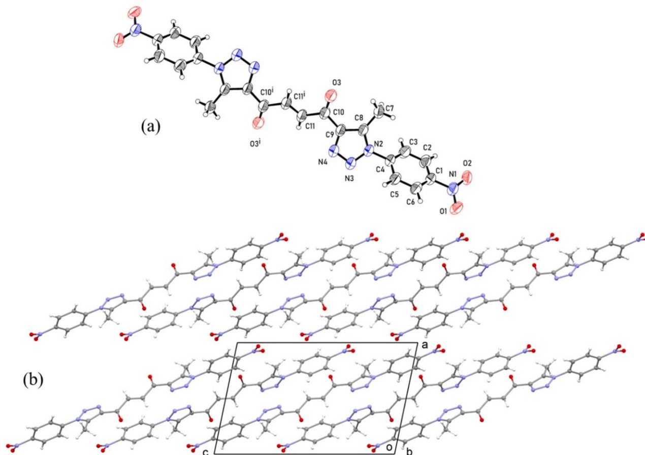
Fig. 1. (a) An ortep representation of 4 showing atomic displacement ellipsoids at 50 % probability and (b) crystal packing viewed along the b axis.
