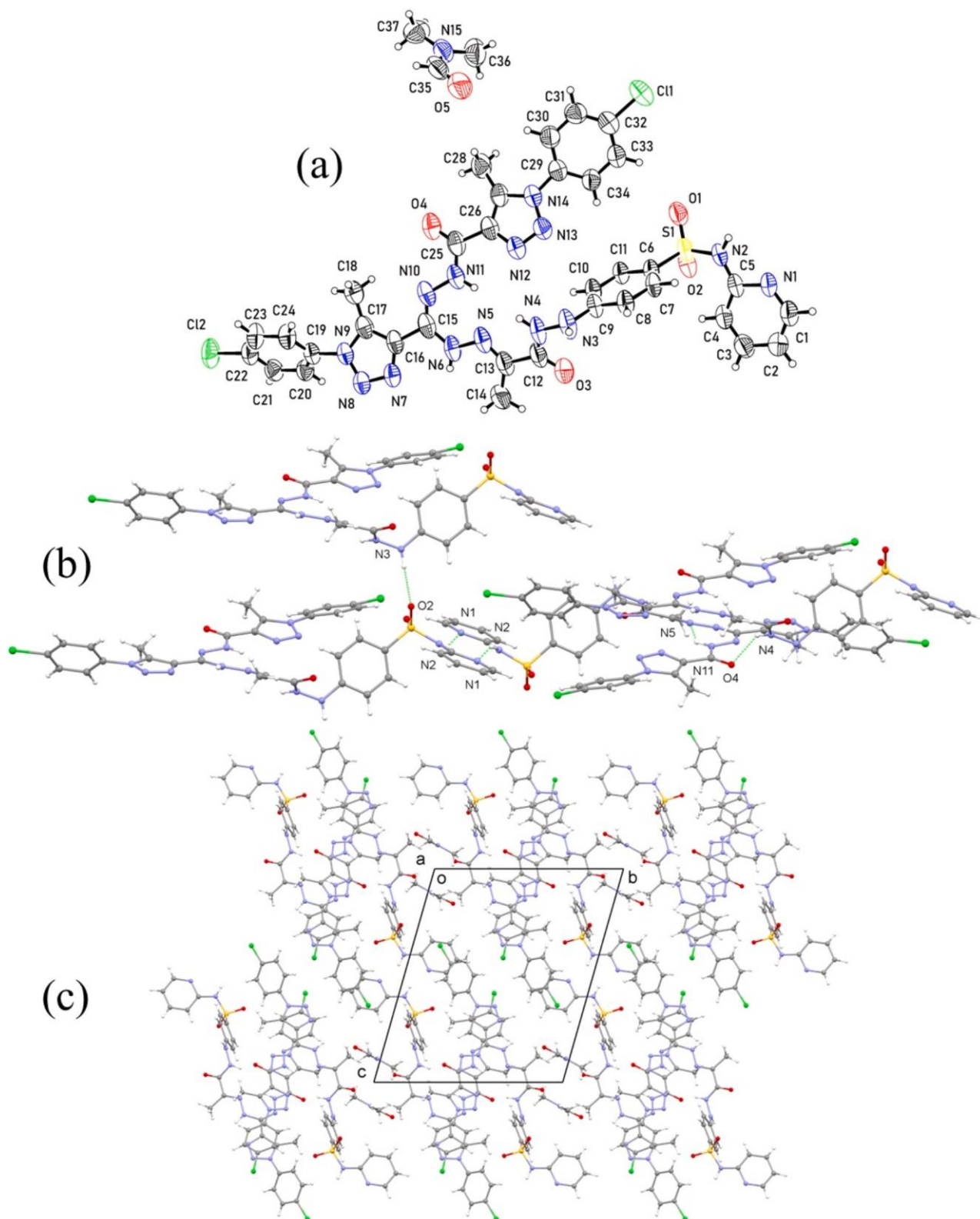
Fig. 5. (a) The asymmetric unit of 21 showing atomic displacement ellipsoids at 50 % probability, (b) a segment of the structure showing hydrogen bonding contacts as green dotted lines and (c) crystal packing viewed along the a axis.
