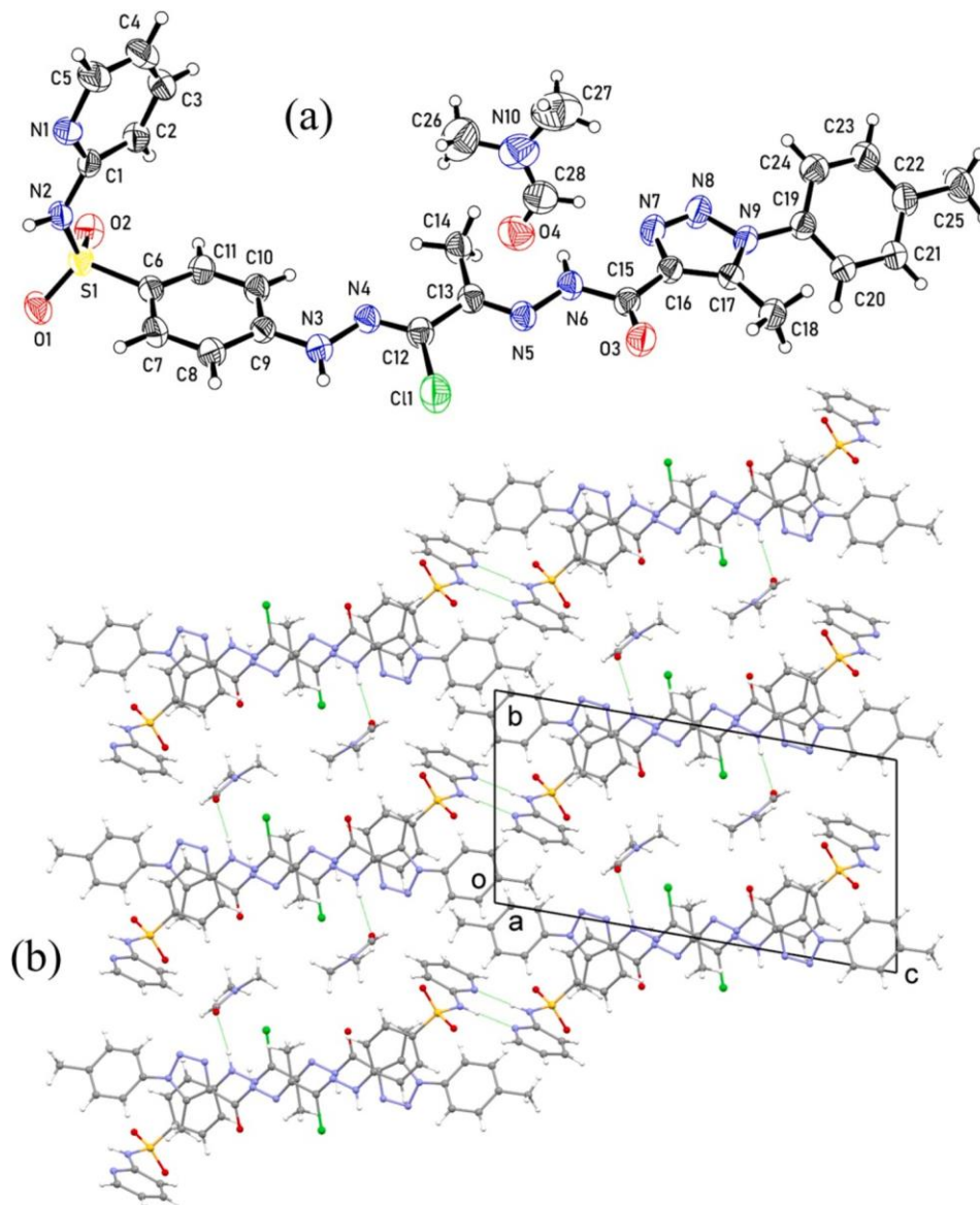
Fig. 4. (a) The asymmetric unit of 20 showing atomic displacement ellipsoids at 50 % probability and (b) crystal packing viewed along the a axis with N–H···O and N–H···N contacts presented as a green dotted line.
