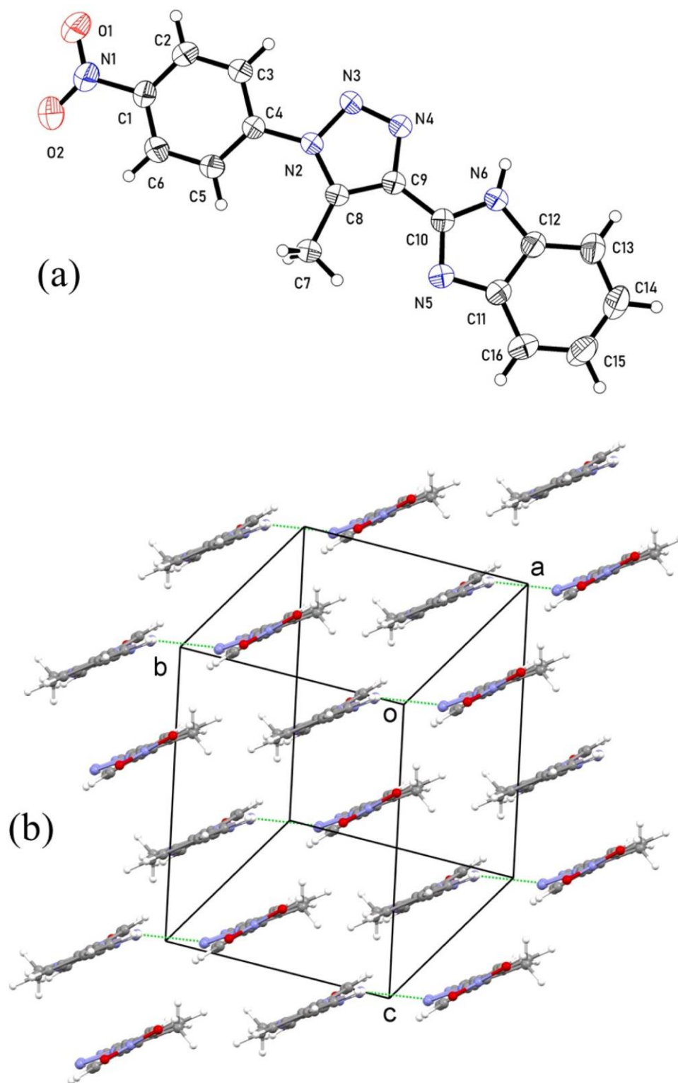
Fig. 2. (a) An ortep representation of 8 showing atomic displacement ellipsoids at 50 % probability and (b) crystal packing viewed along the molecular axis with N–H···O contacts shown as dotted lines.
