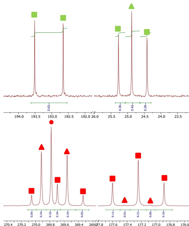
Fig. 16 ^{13}\text{C} containing products from the reaction between 4^{\text{Mes-}13}\text{C} and CO. Top, signals for 8 . Bottom, signals for 2^{\text{Mes}} . Circles signify ^{12}\text{C} products, triangles signify mixed ^{12}\text{C}/^{13}\text{C} and square signifies ^{13}\text{C} products. Markers in green are for ketene ( 8 ) and markers in red are squaraine ( 2^{\text{Mes}} ).
