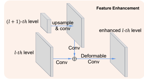
Figure 5: Illustration of the feature enhancement module. The l -th feature level is fused with the upsampled (l+1) -th level by addition, and the fused feature is processed by a deformable convolution.
