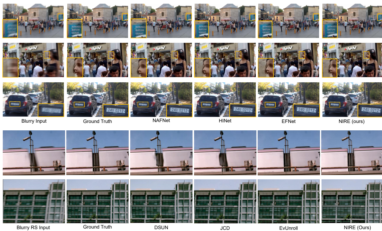
Figure 6: Qualitative result of NIRE dealing with degraded images. For optimal viewing, please zoom in.
