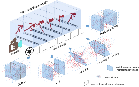
Figure 1: The image re-exposure method adjusts the spatial-temporal domain represented by the image to an expected states, which is able to address issues including deblur, VFI, unrolling, and their combinations with a single model.
