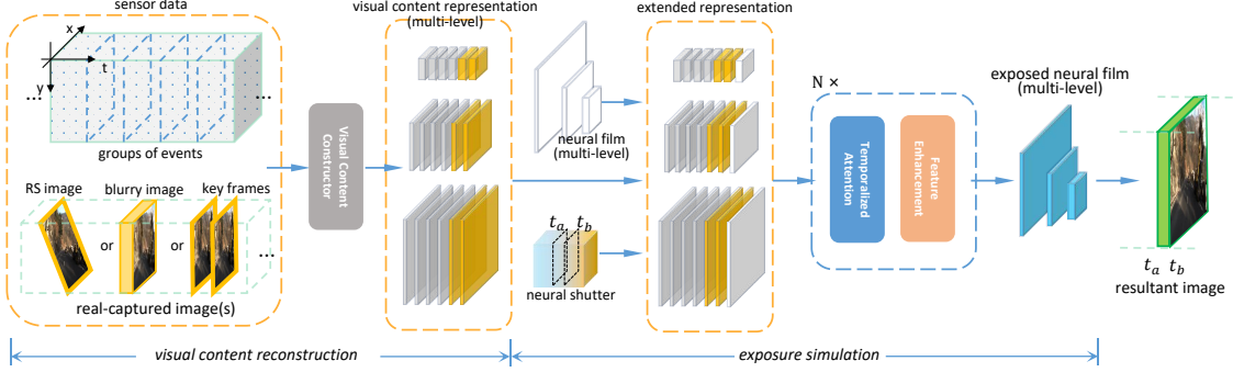
Figure 2: Overall pipeline. A multi-level representation of the visual content is constructed from the sensor data by the visual content constructor. Then, together with the visual content, a multi-level neural film is fed into the exposure simulator. By specifying a desired neural shutter, a desired re-exposed image can be produced.
