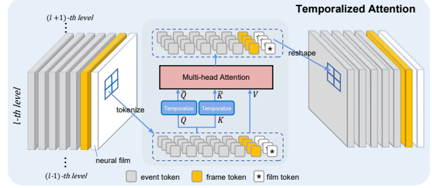
Figure 4: Illustration of the temporalized attention module.
