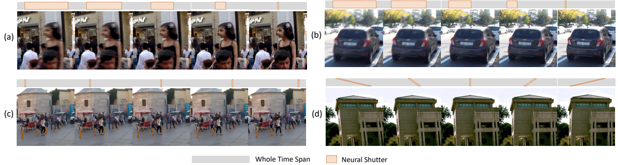
Figure 7: Illustration of the neural shutter and the resulted images. For optimal viewing, please zoom in.
