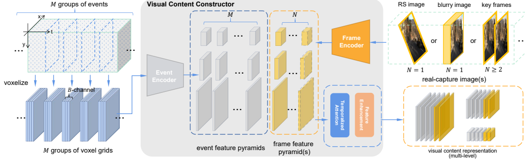
Figure 3: Illustration of the visual content constructor. It first extracts features from events and images, produces a set of multi-level feature pyramids. The feature pyramids are then processed by temporalized attention and feature enhancement, resulting in a multi-level representation of visual content.
