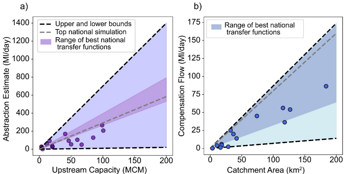
Figure 4. Relationship between (a) reservoir capacity upstream of a gauge and the reservoir abstraction volume (ABS) and 345 (b) catchment area upstream of a gauge and compensation flow (CF). Dots represent data from a sample of catchments where abstractions could be estimated using a water balance hydrological signature and compensation flows could be extracted from Drought Plans, WRMPs and observed downstream flow duration curves (see Section 3.5.1 and Section 1 in Supplementary Material). Grey dashed lines represent the linear transfer functions associated with the top performing simulation from the nationally-consistent calibration, the darker shading represents the spread of the top 5% of nationally-consistent simulations 350 and black dashed lines represent the limits of the transfer function parameters based on the sensitivity of model performance to these parameters (see Table S1 and Section 2 in the Supplementary Material).
