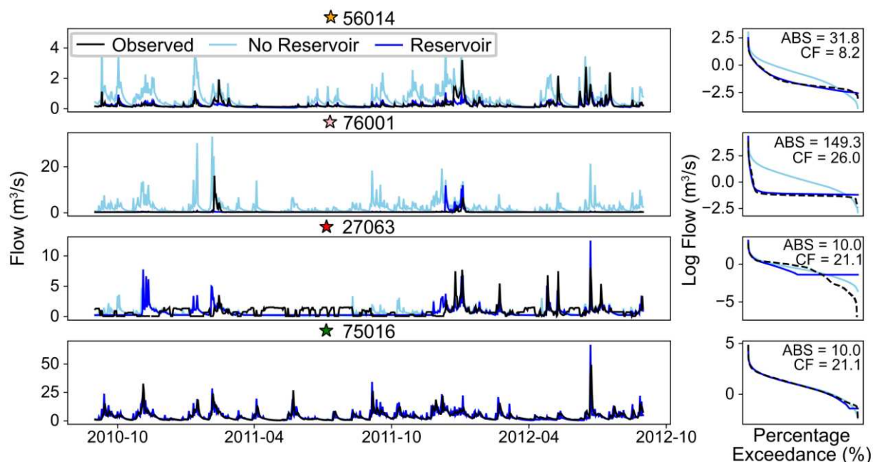
Figure 7. Hydrographs and flow duration curves from the best individual simulations (catchment-by-catchment) for selected reservoir catchments. CF and ABS are recorded on each catchments flow duration curve in MI/day.
