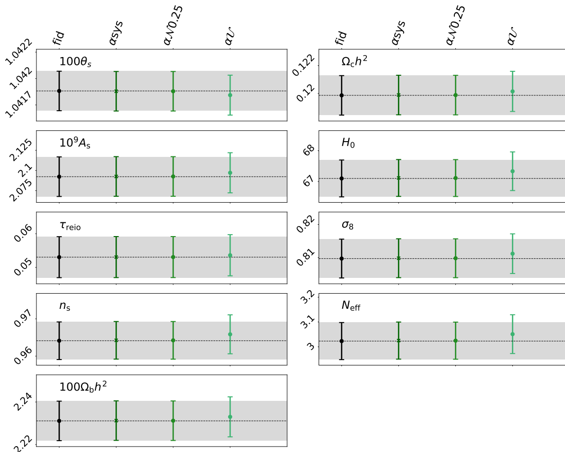
Figure 6. Average over 100 simulations of the mean values and 1\sigma limits of the cosmological parameters recovered in all polarization angles runs (labels as listed in table 2). The black dashed line indicates the mean value of the benchmark fid case, i.e. \Lambda CDM+ N_{\text{eff}} with \alpha^\nu and the other systematics fixed to the fiducial values. The gray band corresponds to its 1\sigma limit. The cases with mismatches in \alpha are indicated with a cross marker instead of a dot for the mean value. The cases in which \alpha^\nu has an offset of \sim 0.25^\circ (second column) or is marginalized over with \sigma = 0.25^\circ (third column) do not cause relevant biases, meaning that a level of \sim 0.25^\circ uncertainty on \alpha^\nu is acceptable for the SO LAT. Noticeable biases instead appear in cosmological parameters, especially a 0.36\sigma shift in N_{\text{eff}} , when we marginalize over \alpha^\nu with a flat prior (last column; described in section 5.2.2). This is due to the fact that the posteriors of \alpha^\nu peak around 1^\circ (see figure 10) causing much larger corrections in the model.
