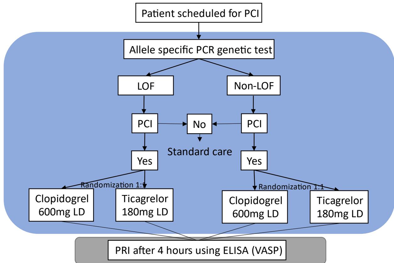
Fig 1. Flow Chart Summary of the study. PCR: Polymerase chain reaction; LOF: Loss of function; NMR: Nuclear magnetic resonance; LD: Loading dose; PRI: Platelet reactivity index; PCI: percutaneous coronary intervention; VASP: vasodilator-associated stimulated phosphoprotein. Note: lack of interaction between ethnicity and both LOF alleles and PRI.
