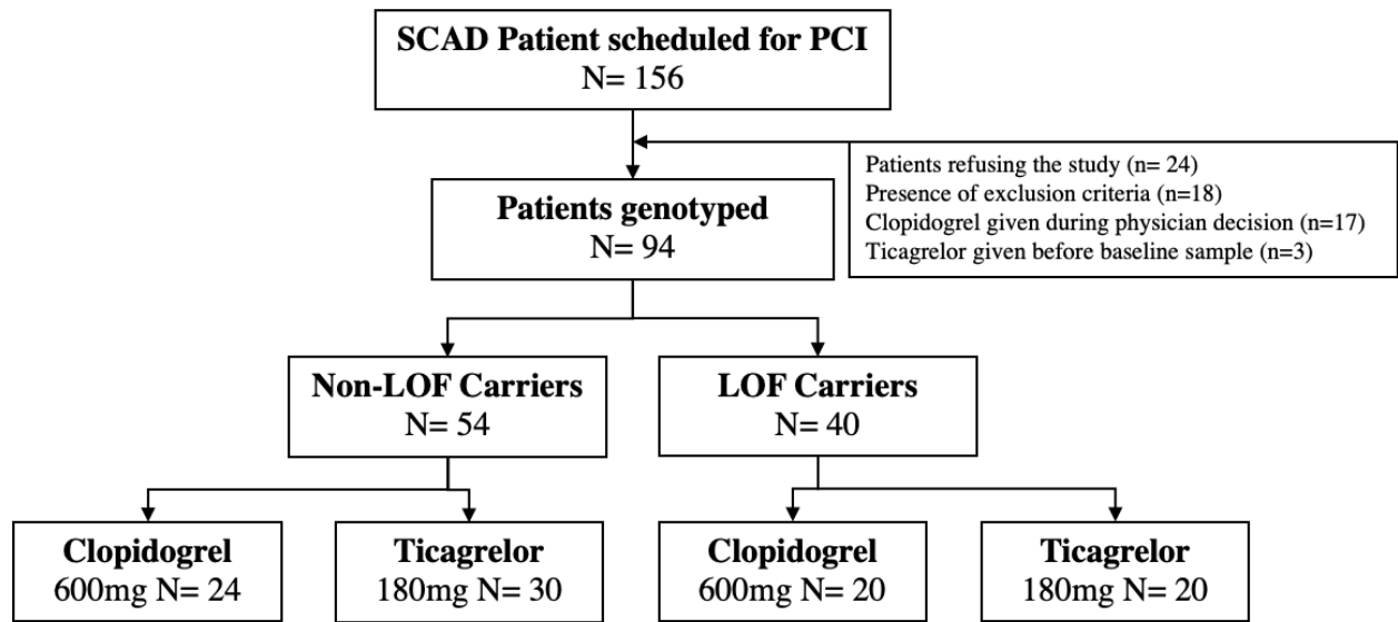
Fig 2. The population of the study. SCAD: Stable coronary artery disease; LOF: Loss of function; LD: Loading dose; PCI: Percutaneous coronary intervention. Note: lack of interaction between ethnicity and both LOF alleles and PRL
