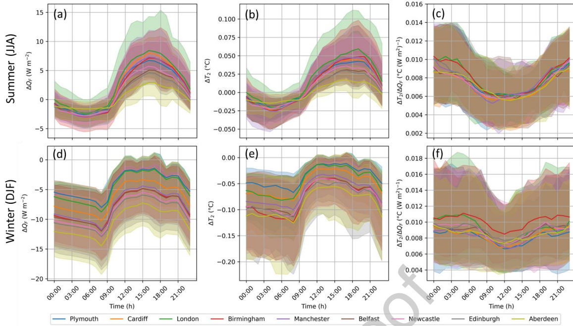
Fig. 14. Median (line) and 5 th and 95 th percentiles (shading) for (a) increases in anthropogenic heat emission ( \Delta Q_{F,B} ), (b) increases in 2 m air temperature ( \Delta T_2 ) and (c) \Delta T_2/\Delta Q_{F,B} in summer (JJA) by replacing gas boilers with ASHPs for different UK locations in the 2050s design summer year.
