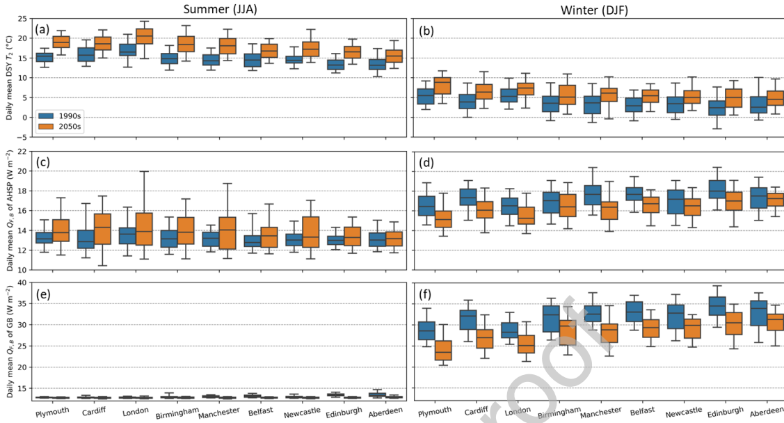
Fig. 12. For flats in UK cities (with increasing latitude, Fig. 4c) under 1990s and 2050s (colour) for (a,c,e) summer (JJA) and (b,d,f) winter (DJF) climate, the variability of the daily mean (a, b) 2 m DSY air temperature ( T_2 ) (monthly values shown in Fig. 4a, b), (c, d) anthropogenic heat emissions ( Q_{F,B} ) from ASHP, and (e, f) Q_{F,B} from gas boilers. Median (horizontal line), interquartile range (box), and 5 th and 95 th percentiles (whiskers) shown. London 2050s Q_{F,B} results given in Fig. 5b.
