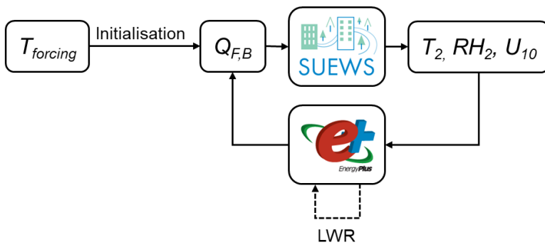
Fig. 2. Model workflow showing the feedback loop between building heat emissions Q_{F,B} and outdoor air temperature T_2 . LWR: inter-building longwave radiation modelling (Xie et al., 2022).
