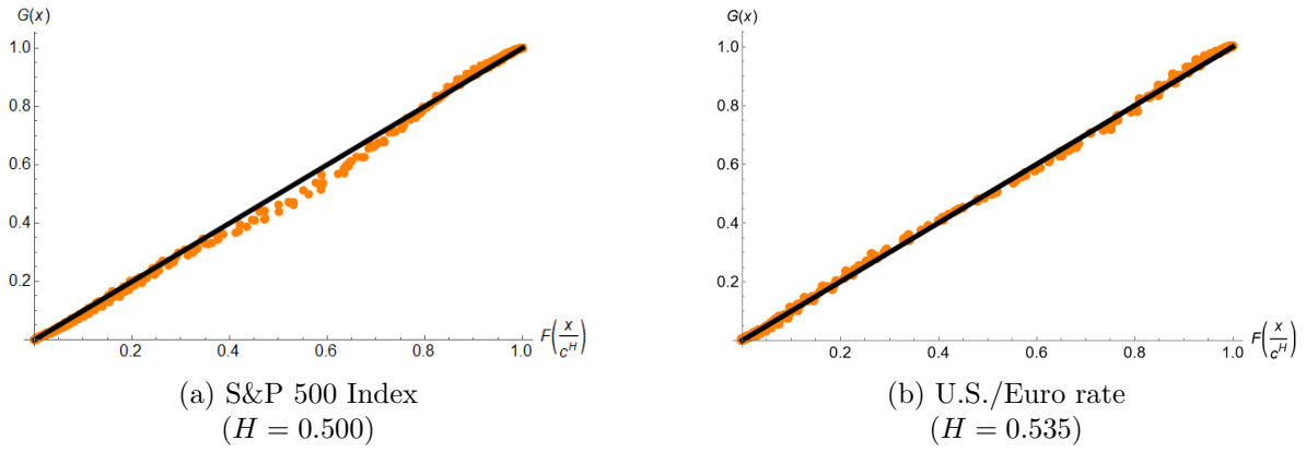
Figure 2: Asymptotic self-similarity of returns
