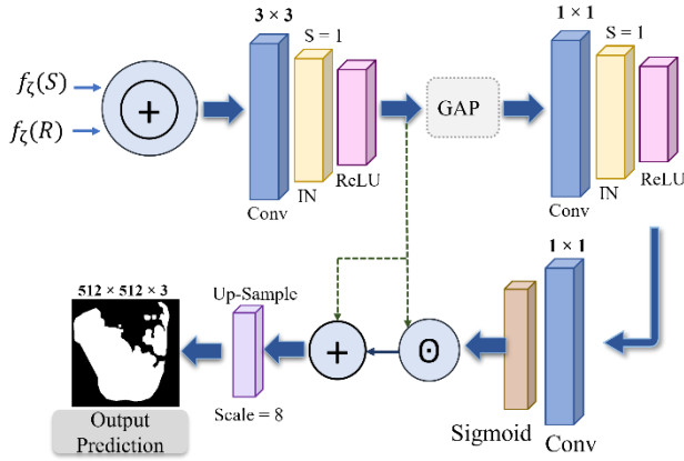
Fig. 5. Fusion module of proposed network, which performs the fusion of the outputs from the SSN and CSN.
