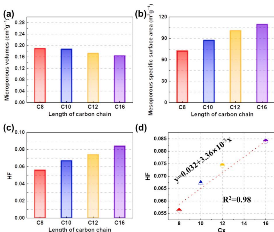
Fig. 3. (a) The microporous volumes, (b) mesoporous specific surface area and (c) HF of titanosilicalites synthesized by surfactants with different carbon chains (i.e., C8, C10, C12 and C16), (d) the linear relationship between the HF of different titanosilicalites and length of carbon chains.
