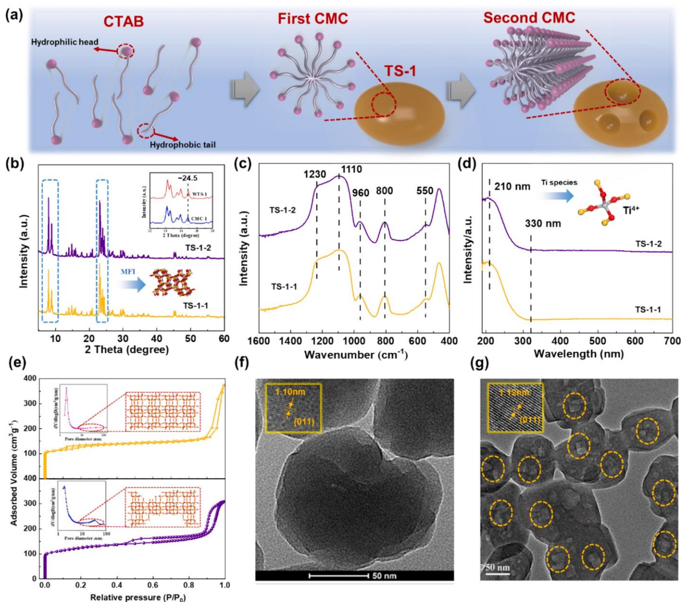
Fig. 1. (a) The schematic diagram of self-assembled structure at different CTAB concentrations. (b) The XRD patterns, (c) FT-IR spectra, (d) UV-vis spectra of different titanosilicalites at first CMC (TS-1-1) and second CMC (TS-1-2). The nitrogen adsorption isotherms of (e) TS-1-1 and TS-1-2 catalysts. The typical HRTEM images of (f) TS-1-1 and (g) TS-1-2 catalysts.
