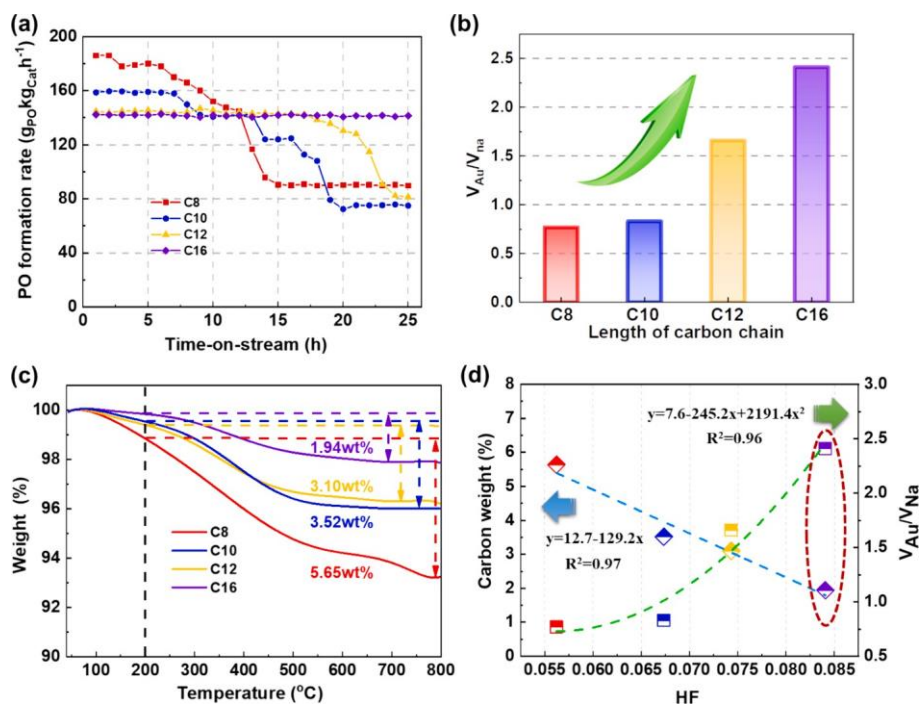
Fig. 4. (a) The PO formation rate with different catalysts at time-on stream, (b) the V_{Au}/V_{Na} and (c) TG profiles of different catalysts after propene epoxidation with H_2 and O_2 for 25 h, (d) the relationship between the HF, carbon content and V_{Au}/V_{Na} .
