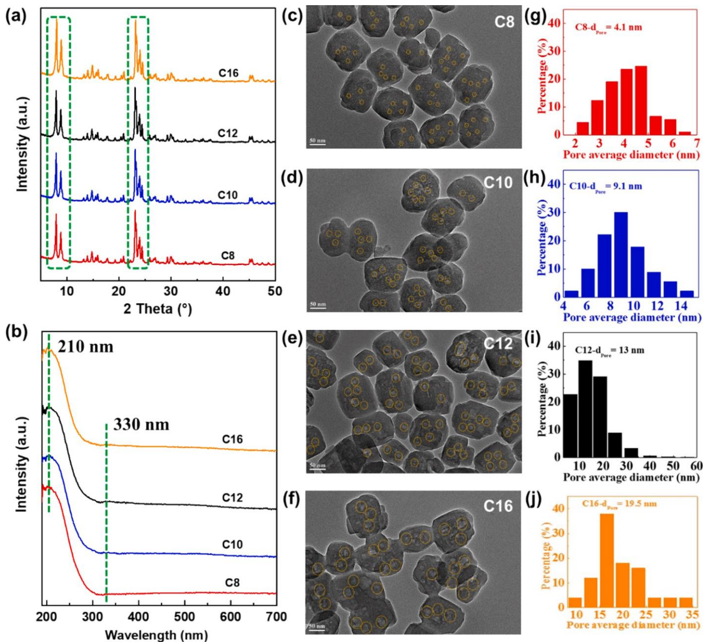
Fig. 2. (a) The XRD patterns and (b) UV-vis spectra of different titanasilicalites synthesized by surfactants with different carbon chains (i.e., C8, C10, C12 and C16). The typical TEM images of titanasilicalites synthesized by (c) C8, (d) C10, (e) C12, and (f) C16 surfactants. The pore average diameter of titanasilicalites synthesized by (g) C8, (h) C10, (i) C12, and (j) C16 surfactants.
