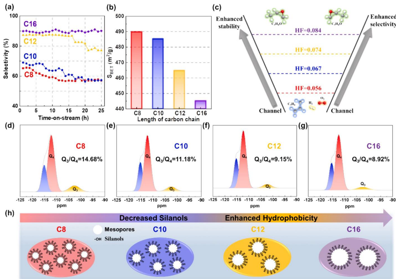
Fig. 5. (a) The PO selectivity with different catalysts at time-on stream, (b) the BET surface area of different titanosilicates, (c) the schematic diagram of the relationship between the regulated diffusion described by the HF and the reaction performance, the 29 Si MAS NMR spectra of (d) MTS-1-C8 (e) MTS-1-C10 (f) MTS-1-C12 (g) MTS-1-C16 supports, and (h) the schematic diagram of the silanols in the different titanosilicates.
