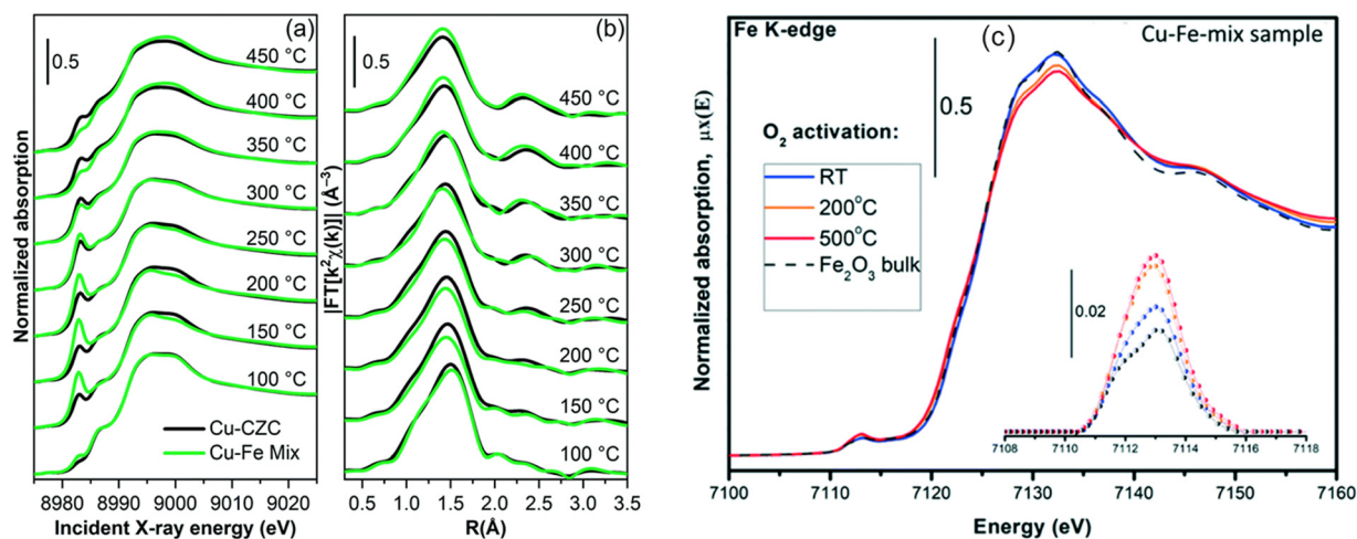
Fig. 16 Cu and Fe speciation in \text{NH}_3 -SCR catalysts (a) normalized Cu K-edge XANES spectra, (b) k^2 -weighted phase-uncorrected FT of EXAFS spectra at various temperatures under \text{NH}_3 -SCR conditions, comparing the monometallic Cu-CZC (black) and bimetallic Cu-Fe-mix (green) catalysts, and (c) Fe K-edge XANES spectra for the Cu-Fe-mix catalyst at RT, 200 °C, and 500 °C after oxygen activation, compared to bulk \alpha - \text{Fe}_2\text{O}_3 (dashed line). The inset shows a magnified view of the background-subtracted pre-edge peak. Reproduced from ref. 269 with permission from The Royal Society of Chemistry, copyright 2024.
