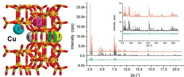
Fig. 8 Rietveld refinement plots illustrating the dehydrated H_{1.99}Cu(I)_{2.37}-Cu(II)_{0.00}MFI phase at room temperature ( 25\text{ }^{\circ}C ) are presented. The plots include observed profiles (in the middle, shown in black), calculated profiles (above, depicted in red), and difference profiles (below, represented in green). These plots were generated using X-ray synchrotron radiation with a wavelength of \lambda = 0.50013\text{ \AA} . The fitting parameters R_p/R_{wp}/R_{exp}/R_1 = 7.3/8.4/5.8/6.2\% . The populations of Cu1/Cu2/Cu2'/Cu3/Cu3' within a unit cell are 0.0/1.07/0.02/0.17/0.45 and 0.18/1.12/0.44/0.20/0.50 , respectively. Reproduced from ref. 211 with permission from American Chemical Society, copyright 2007.
