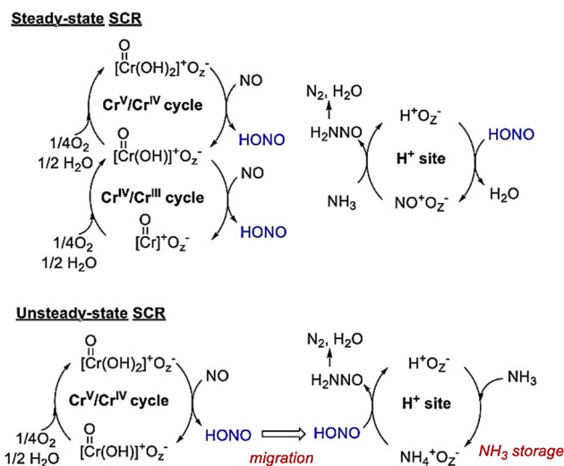
Fig. 21 Mechanism of \text{NH}_3 -SCR Catalyzed with Cr-zeolite catalysts in the steady-state (top) and unsteady-state (bottom) in which the mobile HONO intermediate migrates and reacts with the adsorbed \text{NH}_3 . Reproduced from ref. 17 with permission from American Chemical Society, copyright 2015.
