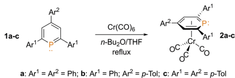
Scheme 1 Synthesis of phosphinine-Cr(CO) 3 -π-complexes 2a–c .
