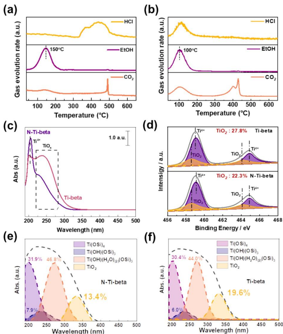
Fig. 2. TG-MS analysis results of (a) ammonia-regulated and (b) conventional Ti precursor supported on dealuminized Beta. (c) UV-vis spectra of hydrolyzed ammonia-regulated and conventional hydrolyzed Ti precursor. (d) XPS analysis of N-Ti-beta and Ti-beta samples in Ti(2p) regions. Diffuse reflectance (DR) UV-vis spectra of (e) ammonia-regulated N-Ti-beta and (f) conventional Ti-beta samples.
