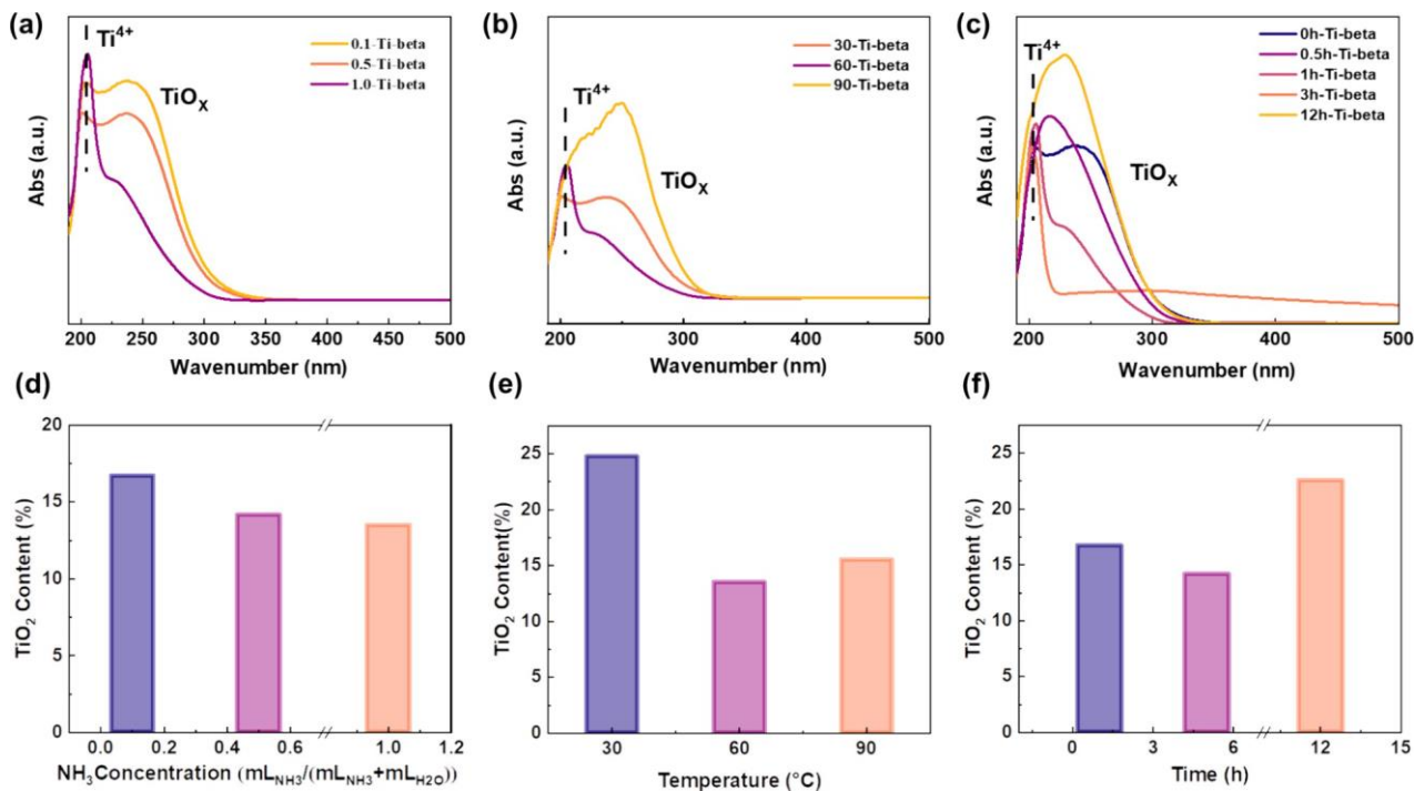
Fig. 5. UV-vis spectra of hydrolyzed ammonia-regulated Ti precursors at (a) different ammonia concentration, (b) different pretreatment temperatures (30 ^{\circ}\text{C} , 60 ^{\circ}\text{C} and 90 ^{\circ}\text{C} ) and (c) different pretreatment time (0, 0.5, 1, 3 and 12 h). \text{TiO}_2 contents determined by UV-vis spectra in Ti-beta pretreated at (d) different ammonia concentration, (e) different pretreatment temperatures and (f) different pretreatment time.
