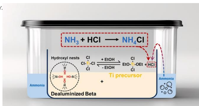
Fig. 1. The schematic diagram of ammonia-regulated evolution of Ti precursor and further incorporation into the framework of dealuminized Beta.
