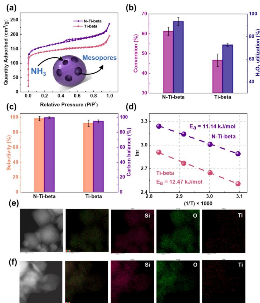
Fig. 3. (a) The N 2 adsorption–desorption isotherms of ammonia-regulated N-Ti-beta and conventional Ti-beta samples. (b) and (c) Catalytic reaction performances in 1-hexene epoxidation with ammonia-regulated N-Ti-beta and conventional Ti-beta samples. Reaction conditions: catalyst (0.2 g), CH 3 CN (20 mL), H 2 O 2 (30 wt%, 1.2 g), 1-hexene (1.2 g), reaction temperature (60 °C), reaction time (3 h), stirring rate (300 rpm). (d) Arrhenius plots over ammonia-regulated N-Ti-beta and conventional Ti-beta samples. The TEM-mapping of Si, O and Ti elements in (e) ammonia-regulated N-Ti-beta and (f) conventional Ti-beta samples.
