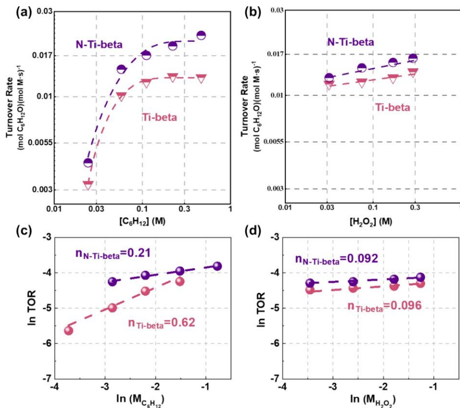
Fig. 4. Turnover rate for 1-hexene epoxidation over ammonia-regulated N-Ti-beta and conventional Ti-beta catalysts as a function of (a) 1-hexene and (b) \text{H}_2\text{O}_2 concentration. Prediction of kinetic reaction order for (c) 1-hexene and (d) \text{H}_2\text{O}_2 over ammonia-regulated N-Ti-beta and conventional Ti-beta catalysts.
