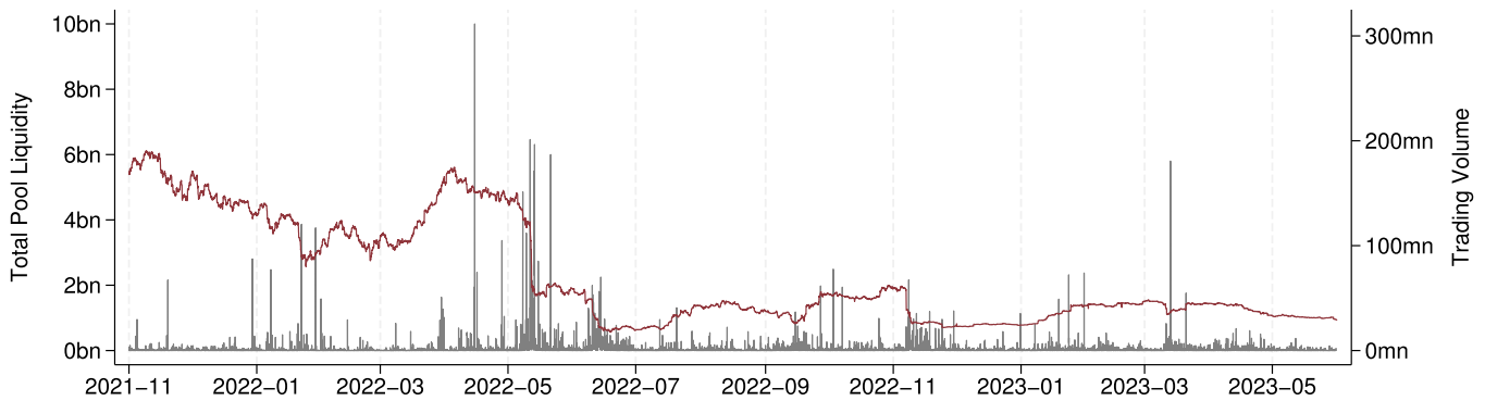
FIGURE 2 | Liquid staking basis and DEX pool dynamics. Note: These graphs show the hourly development of the stETH-ETH liquidity pool at the decentralized exchange Curve. Panel A shows the signed liquid staking basis based on transactions in the pool. The gray line shows the price of Ether in USD taken from the Exchange Kraken. Panel B shows the total liquidity available in the pool in USD and the hourly trading volume. [Color figure can be viewed at wileyonlinelibrary.com ]
