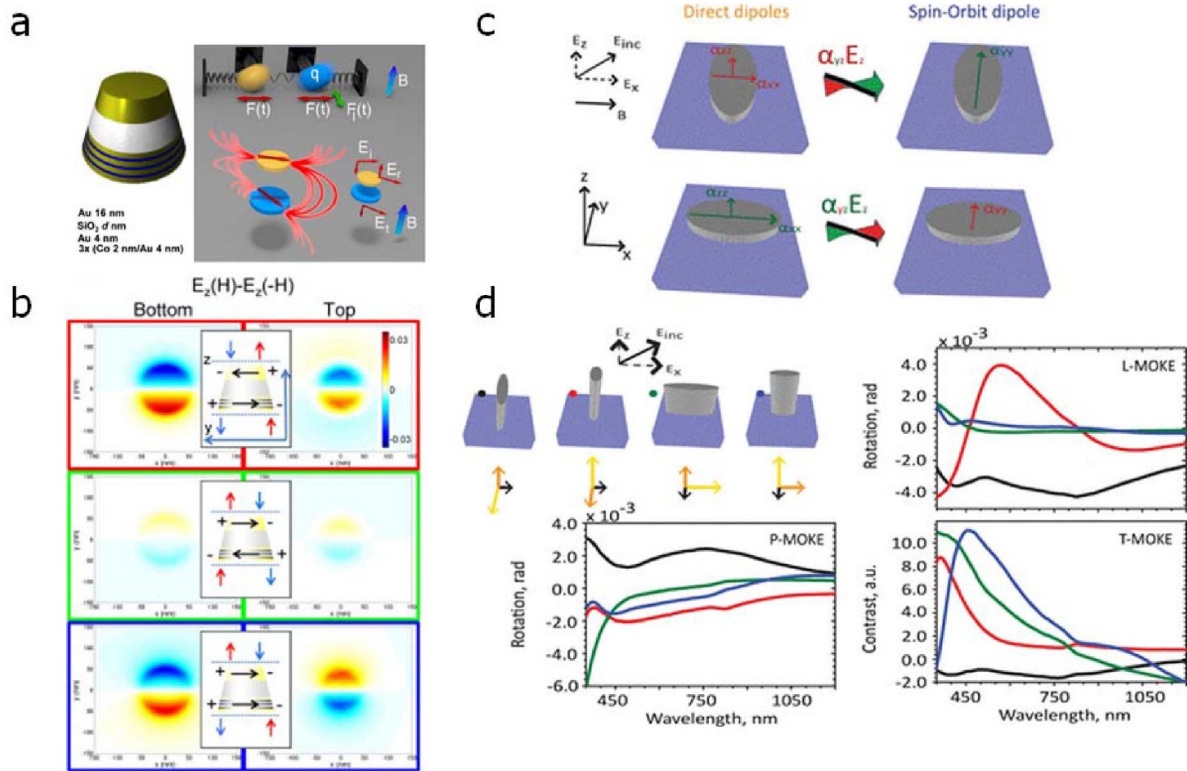
Figure 16. (a) Left panel: schematic drawing of the nanoantennas composed of a purely plasmonic Au disk and a magnetoplasmonic Au/Co superlattice disk separated by a dielectric spacer. Top-right panel: spring model representing a two coupled masses system excited by a harmonic force, F(t) , along x axis. One of the masses (blue) is charged ( q ) and a static magnetic field ( B ) is applied along the z direction, inducing a Lorentz force, F_1(t) , along the y direction. The y -movement is transferred to the other mass through the coupling. Bottom-right panel: two interacting electric dipoles, representing two metallic disks, excited by an incident beam polarized along the x axis. One of the disks (blue) has magneto-optical activity and a static magnetic field ( B ) applied along the z direction induces a rotation of its electric dipole, which is transferred to the other dipole through the interaction. The rotation modifies the polarization direction of the reflected ( E_r ) and transmitted ( E_t ) light. (b) Difference of the E_z components for magnetic saturation along opposite directions in the same planes and for the same structure. This difference accounts for the effect of the applied magnetic field: the appearance of a dipole along the y direction for both the magnetoplasmonic (intrinsic dipole) and the plasmonic (induced dipole) disks. In both cases, the components for three different wavelengths labelled with different colours (red, green, and blue frames). At specific frequencies (e.g. see green frame) the magneto-optical response is suppressed due to the destructive interference between the two dipoles. (c) Schematic overview of the interplay of the directly excited (left, resonant \alpha_{xx} and off-resonant \alpha_{zz} ) and spin-orbit coupled (right, resonant \alpha_{yy} ) nanoantenna modes that all together deliver exceptional light polarization rotation control. Light incidence ( p -polarized) and applied magnetic field are marked. (d) Schematic set of 3D nanoantennas (top, left) with highlighted dipolar on (yellow, orange)/off (grey) resonance modes. p -polarized light is always used. Calculated Kerr signals for the nanoantennas in panel in L-MOKE (top, right), P-MOKE (bottom, right), and T-MOKE (bottom, left). Panels (a) and (b) are reprinted with permission from [97] © Optica Publishing Group. Panels (c) and (d) are reprinted with permission from [100]. Copyright (2014) American Chemical Society.
