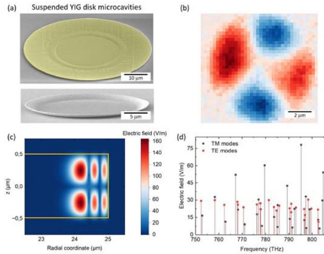
Figure 6. (a) Two suspended YIG disk microcavities, one with a ‘disk on a stem’ structure (diameter of 50\ \mu\text{m} ) and one with a suspended edge structure (diameter of 25\ \mu\text{m} ). The YIG disks are 150\ \text{nm} thick, and their edge is lifted \sim 1\ \mu\text{m} above the GGG substrate. (b) Super Nyquist-sampling magneto-optical Kerr effect (SNS-MOKE) image of a radially symmetric magnon mode in a suspended YIG disk microcavity with a diameter of 7.5\ \mu\text{m} . (c) COMSOL simulation of the electric field distribution of a WGM mode in a YIG disk microcavity. (d) WGM spectrum for TM and TE polarized modes in the same cavity.
