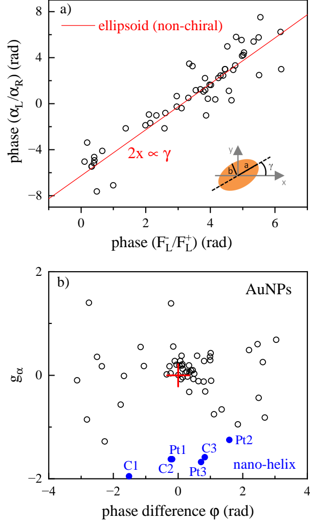
Figure 6: a) Phase of the polarisability ratio \alpha_L/\alpha_R = (F_L^-/F_R^-) \times (F_R^+/F_L^+) versus phase of the cross to co-polarised FWM field ratio F_L^-/F_L^+ , in single nominally spherical AuNPs of 60 nm diameter (same as in Fig. 5). The red line shows the expected dependence assuming a non-chiral quasi-spherical particle of ellipsoidal shape, with in-plane orientation \gamma as sketched in the inset. b) Dissymmetry factor g_\alpha versus the difference between the experimental phase of \alpha_L/\alpha_R and the phase expected from the ellipsoid model. Blue symbols are the results for the nano-helices (using the phase measured at the optimum focus z = 0 , see Fig.3). The centre cross represents the ellipsoid model case.
