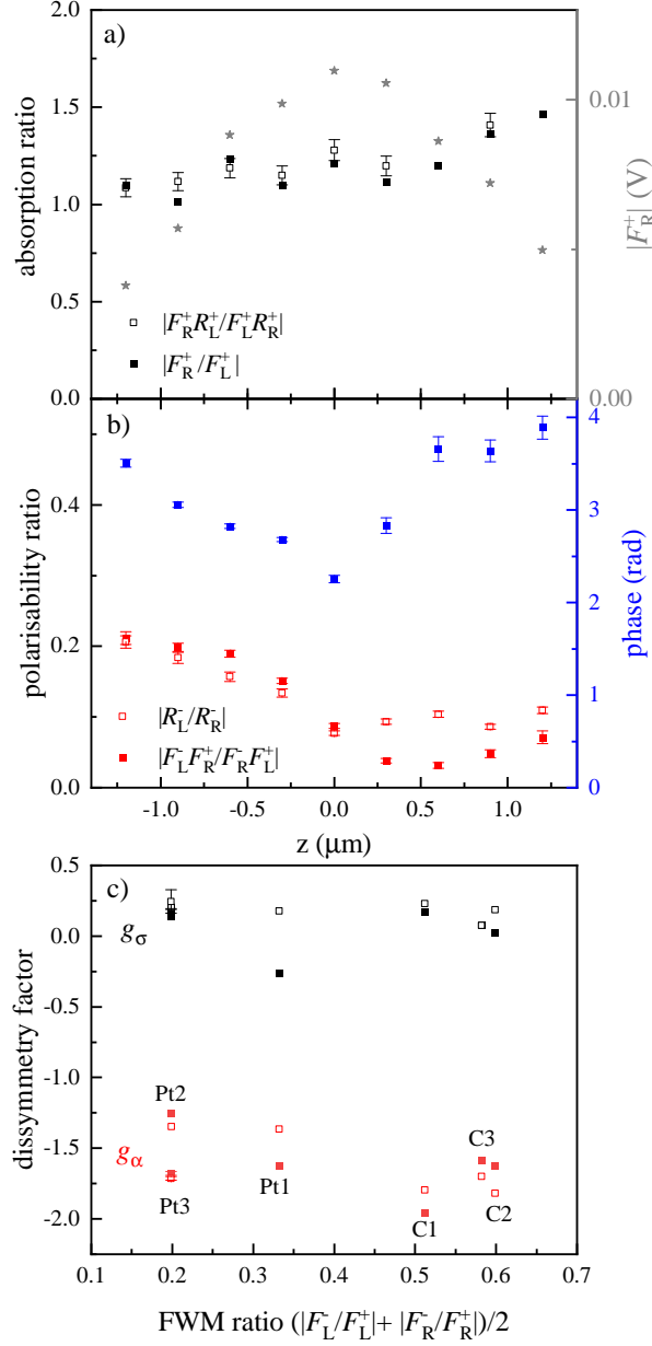
Figure 3: Overview of chiral quantities in single helices. a,b): Dependence on the axial focus position z for the same Pt helix as in Fig. 2. The star symbols with the right axis in a) show the z -dependence of the co-polarised detected FWM field amplitude in the RCP incident probe configuration. The phase in b) refers to the polarisability ratio calculated using \alpha_L / \alpha_R = (F_L^- / F_R^-) \times (F_R^+ / F_L^+) ; absolute phase drifts between the measurements are compensated in the ratio. Error bars are calculated as one standard deviation, from the photon shot-noise and the laser fluctuations in the experiment (see text). When not shown, errors are smaller than the size of the symbols. c): Dissymmetry factors g_\sigma and g_\alpha for all available helices (3 Pt and 3 C) measured at optimum focus versus cross to co-polarised FWM amplitude ratio (average of L and R). Symbols relate the corresponding quantities used to calculate the dissymmetry factor, as per legend in a) and b). The C and Pt helices shown in Fig. 2 correspond to C2 and Pt3. Representative error bars are shown for Pt3.
