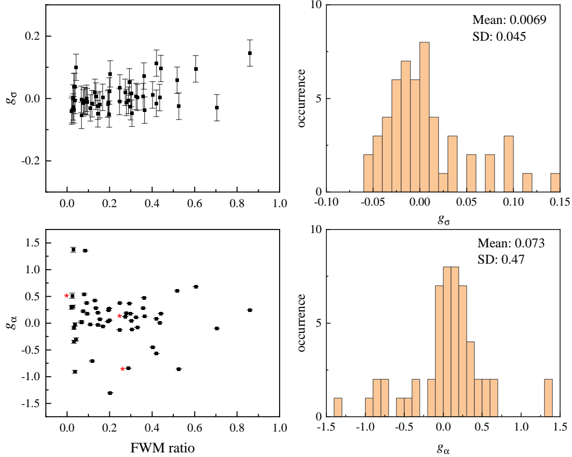
Figure 5: Overview of chiral quantities in single nominally spherical AuNPs of 60 nm diameter. Left: Dissymmetry factors g_\sigma and g_\alpha for all available AuNPs, measured at the spatial location corresponding to the centre of the objective point-spread function for co-polarised FWM, versus cross to co-polarised FWM amplitude ratio (average of L and R). Error bars are calculated as one standard deviation, from the photon shot-noise and the relative laser fluctuations in the experiment (see text). The red stars indicate the 3 AuNPs imaged in Fig. 4. Right: Corresponding histograms of g_\sigma and g_\alpha , with indicated mean and standard deviation (SD).
