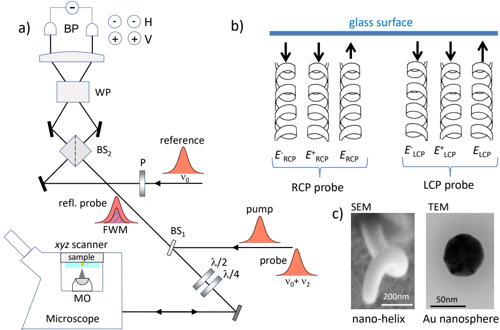
Figure 1: a) Sketch of the experimental set-up with interferometric detection of the FWM field and polarisation-resolved configuration. Pump and probe pulses are coupled into an inverted microscope equipped with a high NA microscope objective (MO). The probe optical frequency \nu_0 is slightly upshifted by a radio frequency amount \nu_2 . Incident beams are adjusted to be circularly polarized at the sample by \lambda/4 and \lambda/2 wave plates. The reflected circular polarizations are transformed into horizontal (H) and vertical (V) linear polarization by the same wave plates, and both components are simultaneously detected through their interference with a frequency unshifted reference linearly polarized at 45 degrees (see text). BP: Balanced photodiodes. WP: Wollaston prism. b) The polarisation of the incident probe field E is adjusted to be left-circular (LCP) or right-circular (RCP) at the sample. The sketch highlights that the collection is in reflection geometry, and that the light helicity is inverted upon reflection. c) Examples of investigated nanostructures; SEM on a single nano-helix (Carbon material) and TEM of a nominally-spherical gold nanoparticle.
