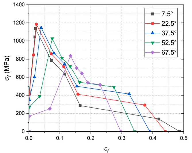
Fig. 12. Stress-strain curves for hooked end steel fibres at various inclinations.
