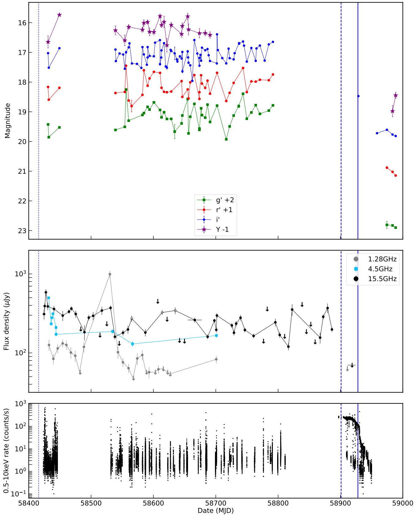
Figure 1. Upper panel: Optical light curves of the J1858 system during outburst and quiescence. Artificial offsets have been placed to make the data easier to visualise. The vertical dotted, dashed and solid blue lines indicate the outburst's beginning, state transition and return to quiescence, respectively. Middle panel: The radio data from van den Eijnden et al. (2020) ; Rhodes et al. (2022) . Lower panel: The 0.5-10 keV NICER light curve from Castro Segura et al. (2022) .
