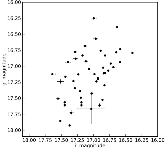
Figure 2. g' vs i' magnitude for observations made within the same night (most are taken within a few minutes during a filter sequence). There is evidence of a correlation but with considerable scatter, indicating that the variability timescale is shorter than the time between observations in different filters.
