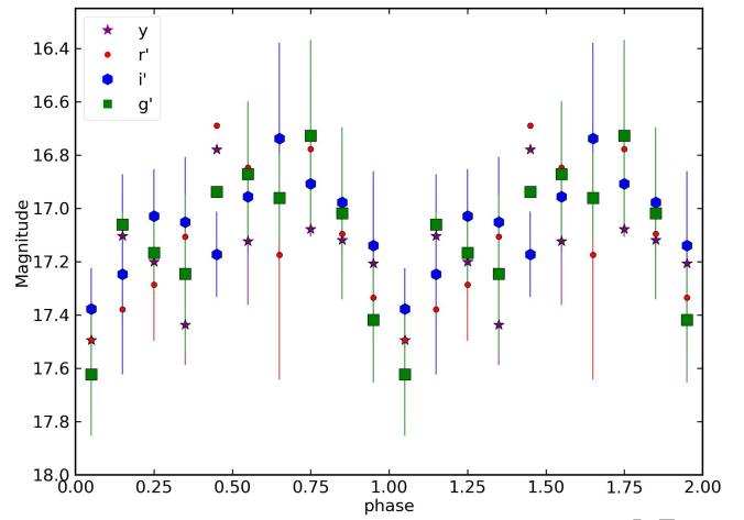
Figure 7. Phase folded light curve for our optical data during the outburst. Each phase bin is 10% of the phase. The uncertainties on each data point reflect the scatter within that phase bin. Points with no error bars only have one observation within that phase bin.
