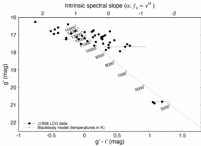
Figure 6. Colour magnitude diagram of J1858 showing optical brightness g' vs color g'-i' where the bluer colours that correspond to higher spectral indices are shown to the left, and redder colors are shown to the right, overplotted with a simple model of a single temperature blackbody heating up and cooling denoted by the black dotted line labelled with temperature values.
