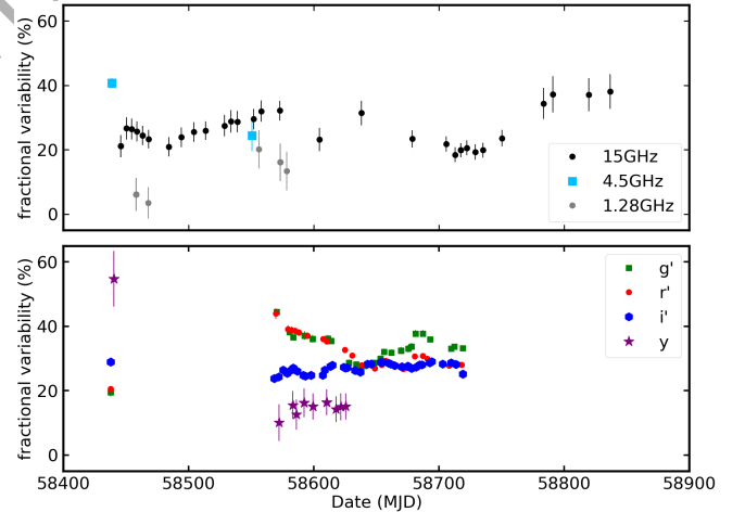
Figure 4. The radio (top panel) and optical (bottom panel) F_{\text{rms}} variability as a function of time. We calculate a moving average rms variability with a bin size of 60 days.
