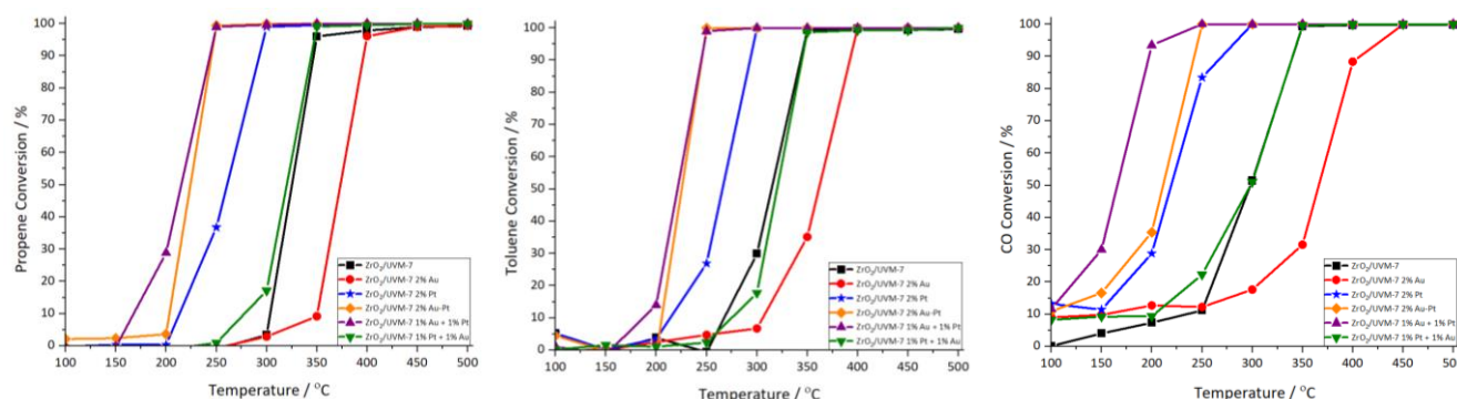
Figure 9: Breakdown of the catalytic activity for the total oxidation of individual pollutants in the mixed gas feed. Propene (Left), toluene (Middle) and CO (Right). Conditions: 100 ppm toluene, 1000 ppm propene, 1000 ppm CO, 6% O 2 /N 2 , WHSV = 60000 mL g -1 h -1 .
