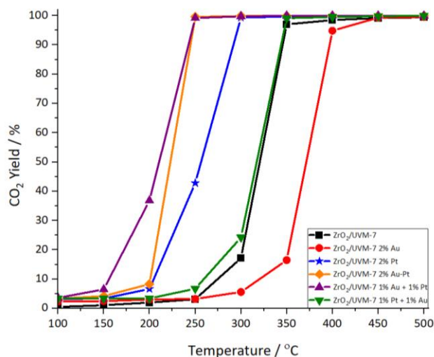
Figure 8: \text{CO}_2 yield acquired for the simultaneous total oxidation of toluene, propene, and CO gas mix. Conditions: 100 ppm toluene, 1000 ppm propene, 1000 ppm CO, 6% \text{O}_2/\text{N}_2 , \text{WHSV} = 60000 \text{ mL g}^{-1} \text{ h}^{-1} . Legend refers to catalysts used.
