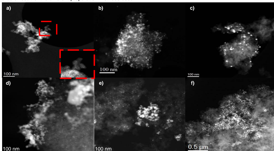
Figure 5: Low magnification Cs-corrected STEM-HAADF images of the calcined catalysts. a) \text{ZrO}_2/\text{UVM-7} b) \text{ZrO}_2/\text{UVM-7} 2% Au c) \text{ZrO}_2/\text{UVM-7} 2% Pt d) \text{ZrO}_2/\text{UVM-7} 2% Au-Pt e) \text{ZrO}_2/\text{UVM-7} 1% Au + 1% Pt f) \text{ZrO}_2/\text{UVM-7} 1% Pt + 1% Au.
