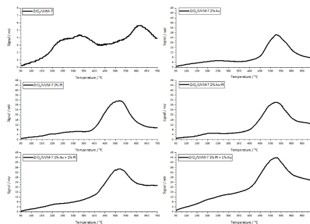
Figure 2: TPR profiles of the calcined catalysts.
