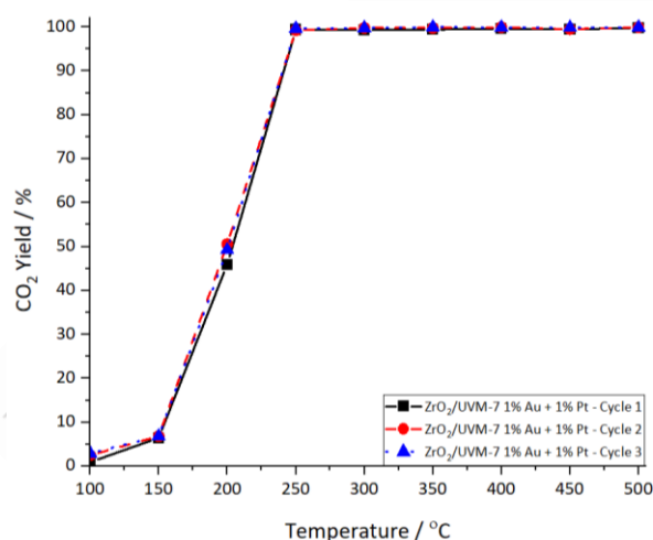
Figure 11: Consecutive cycle tests for the simultaneous total oxidation of toluene, propene and CO using the ZrO 2 /UVM-7 1% Au + 1% Pt catalyst. Conditions: 100 ppm toluene, 1000 ppm propene, 1000 ppm CO, 6% O 2 /N 2 , WHSV = 60000 mL g -1 h -1 . Legend refers to catalyst cycle.
