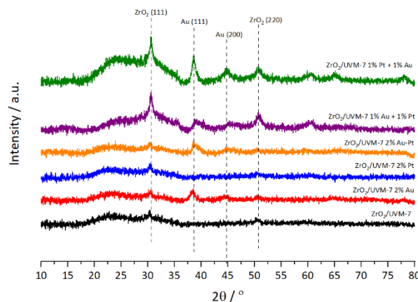
Figure 1: PXRD patterns of the calcined catalysts.
