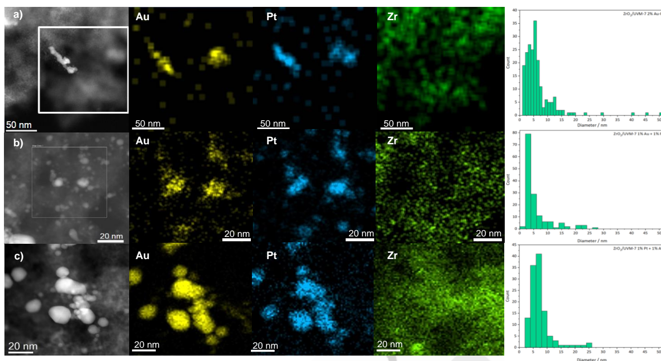
Figure 7: Cs-corrected STEM-HAADF images with corresponding EDX images and particle size histograms for the bimetallic catalyst: a) \text{ZrO}_2/\text{UVM-7} 2% Au-Pt b) \text{ZrO}_2/\text{UVM-7} 1% Au + 1% Pt c) \text{ZrO}_2/\text{UVM-7} 1% Pt + 1% Au.
